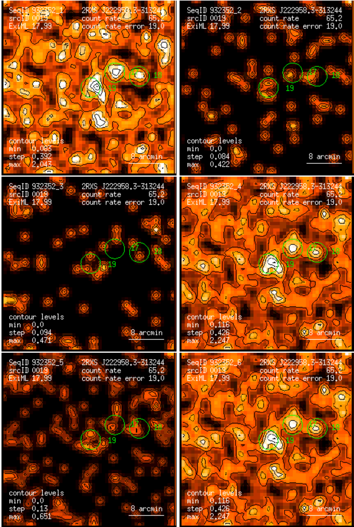
Figure 19: RASS 932352: detection 0019: band rate images, Gaussian filter: (1) PSPC channels 11 – 41, (2) 52 – 90, (3) 91 – 201, (4) 11 – 235, (5) 52 – 201, (6) 11 – 201. Broad band rates in counts/ks. Band rate contour levels in counts/ks/arcmin 2 .
