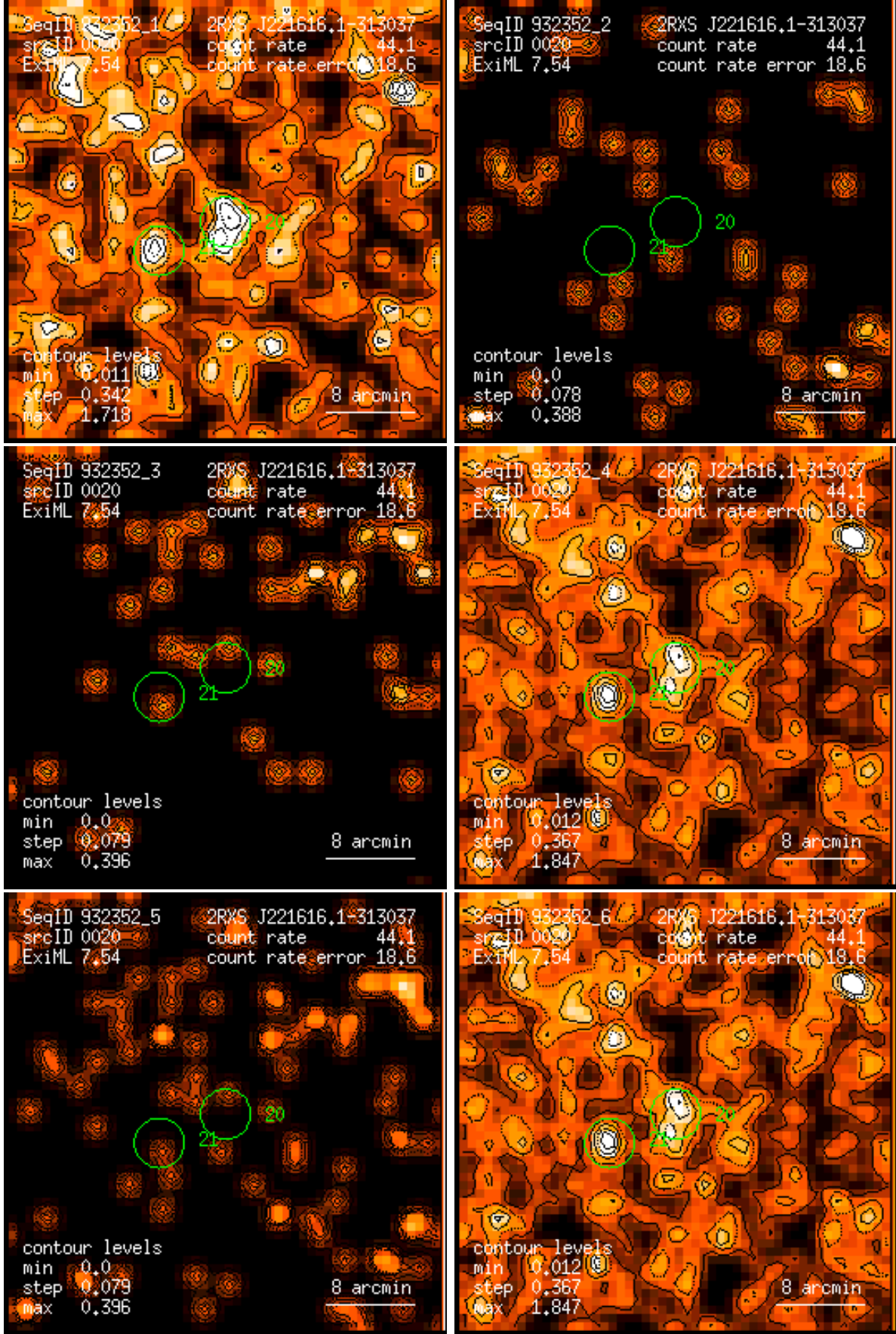
Figure 20: RASS 932352: detection 0020: band rate images, Gaussian filter: (1) PSPC channels 11 – 41, (2) 52 – 90, (3) 91 – 201, (4) 11 – 235, (5) 52 – 201, (6) 11 – 201. Broad band rates in counts/ks. Band rate contour levels in counts/ks/arcmin 2 .
