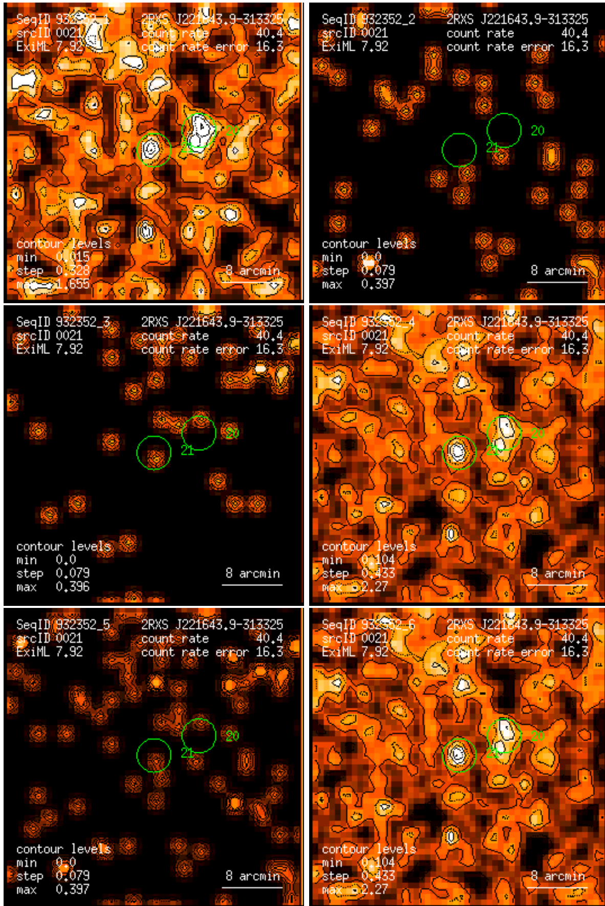
Figure 21: RASS 932352: detection 0021: band rate images, Gaussian filter: (1) PSPC channels 11 – 41, (2) 52 – 90, (3) 91 – 201, (4) 11 – 235, (5) 52 – 201, (6) 11 – 201. Broad band rates in counts/ks. Band rate contour levels in counts/ks/arcmin 2 .
