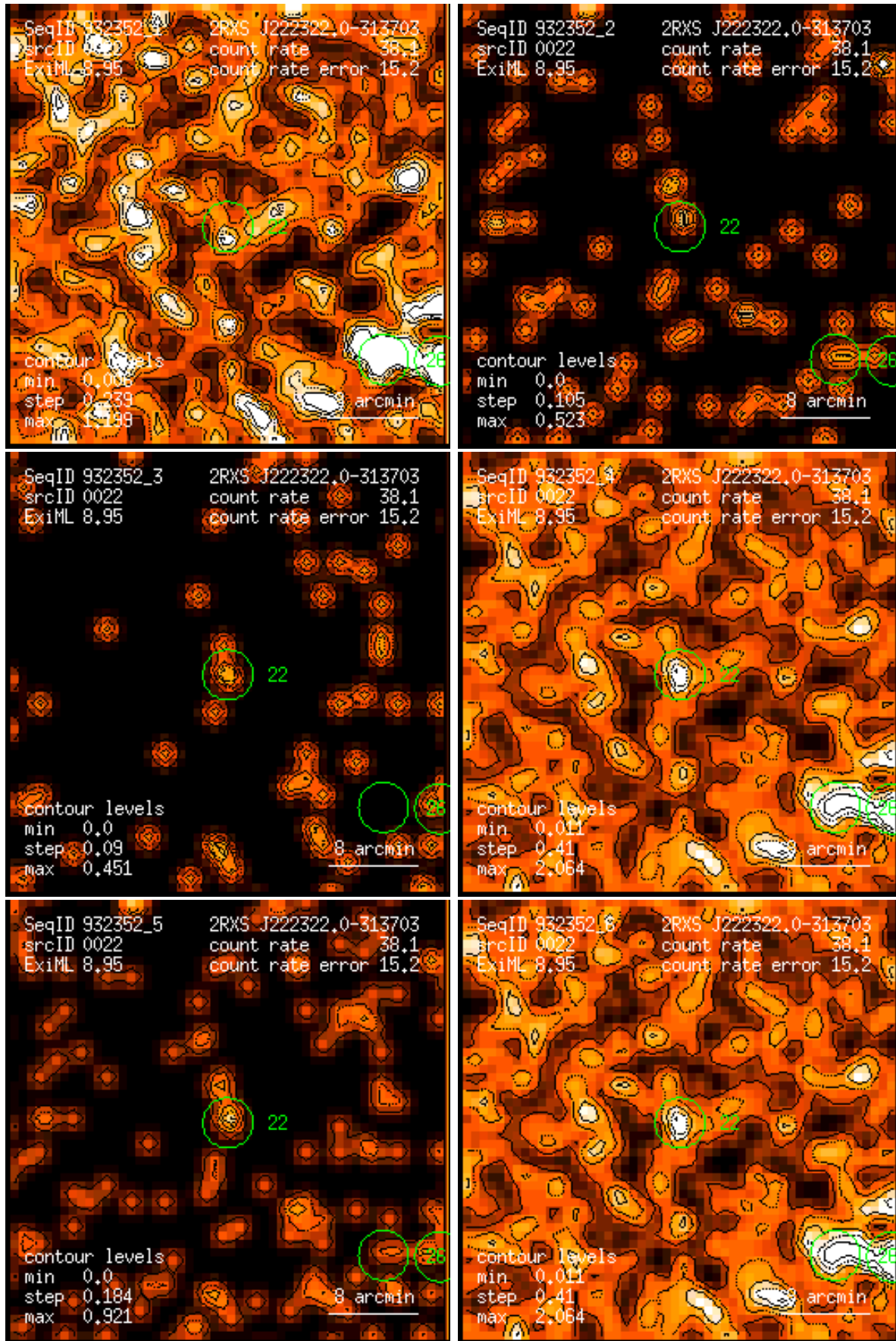
Figure 22: RASS 932352: detection 0022: band rate images, Gaussian filter: (1) PSPC channels 11 – 41, (2) 52 – 90, (3) 91 – 201, (4) 11 – 235, (5) 52 – 201, (6) 11 – 201. Broad band rates in counts/ks. Band rate contour levels in counts/ks/arcmin 2 .
