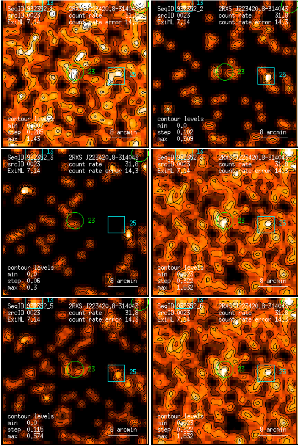
Figure 23: RASS 932352: detection 0023: band rate images, Gaussian filter: (1) PSPC channels 11 – 41, (2) 52 – 90, (3) 91 – 201, (4) 11 – 235, (5) 52 – 201, (6) 11 – 201. Broad band rates in counts/ks. Band rate contour levels in counts/ks/arcmin 2 .
