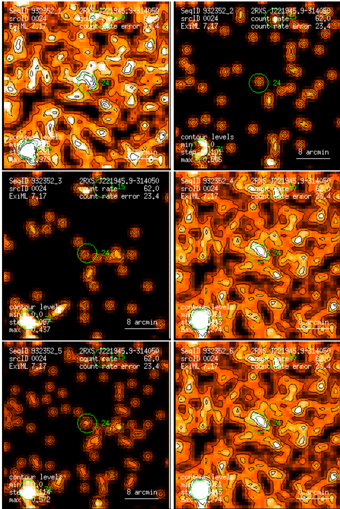
Figure 24: RASS 932352: detection 0024: band rate images, Gaussian filter: (1) PSPC channels 11 – 41, (2) 52 – 90, (3) 91 – 201, (4) 11 – 235, (5) 52 – 201, (6) 11 – 201. Broad band rates in counts/ks. Band rate contour levels in counts/ks/arcmin 2 .
