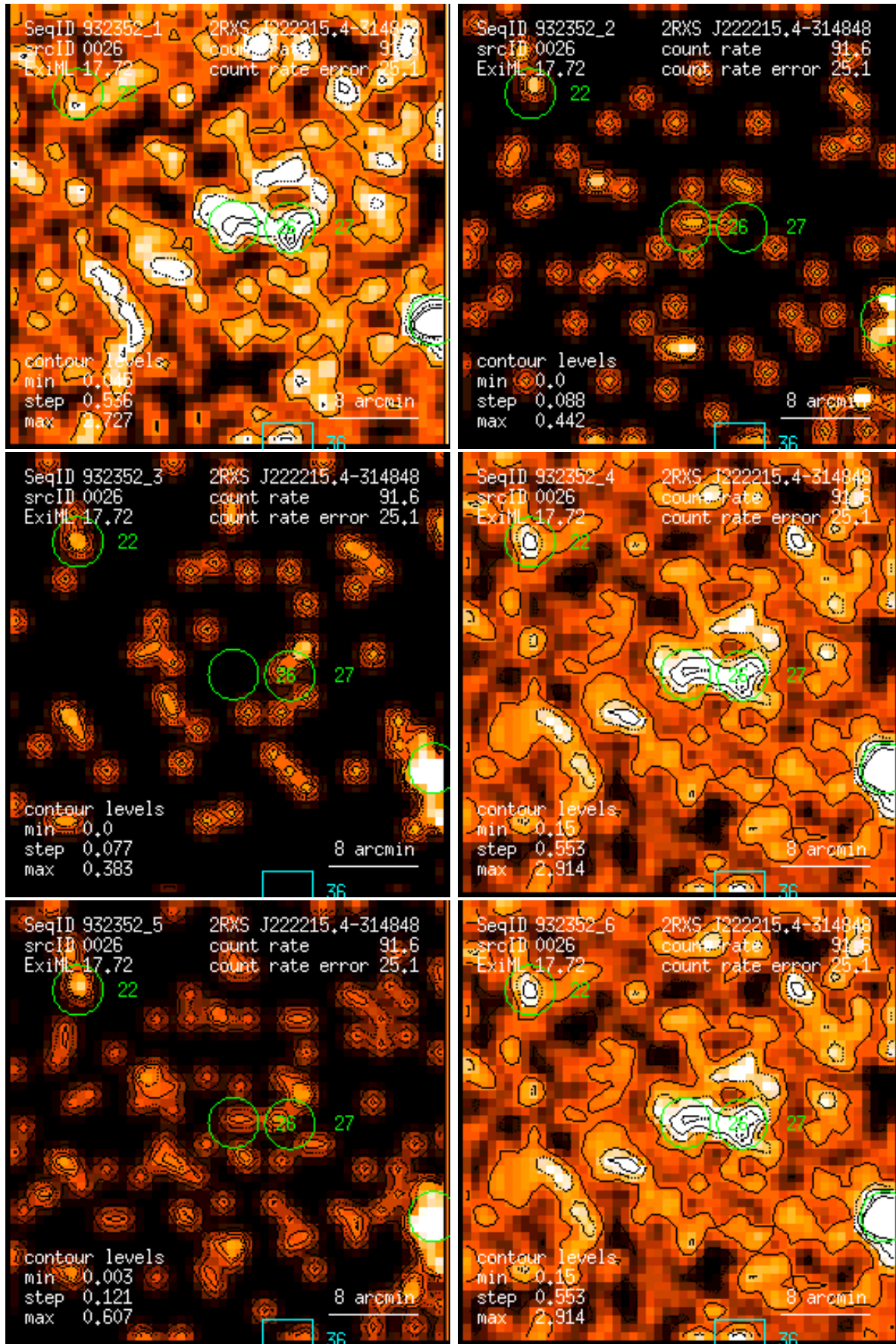
Figure 26: RASS 932352: detection 0026: band rate images, Gaussian filter: (1) PSPC channels 11 – 41, (2) 52 – 90, (3) 91 – 201, (4) 11 – 235, (5) 52 – 201, (6) 11 – 201. Broad band rates in counts/ks. Band rate contour levels in counts/ks/arcmin 2 .
