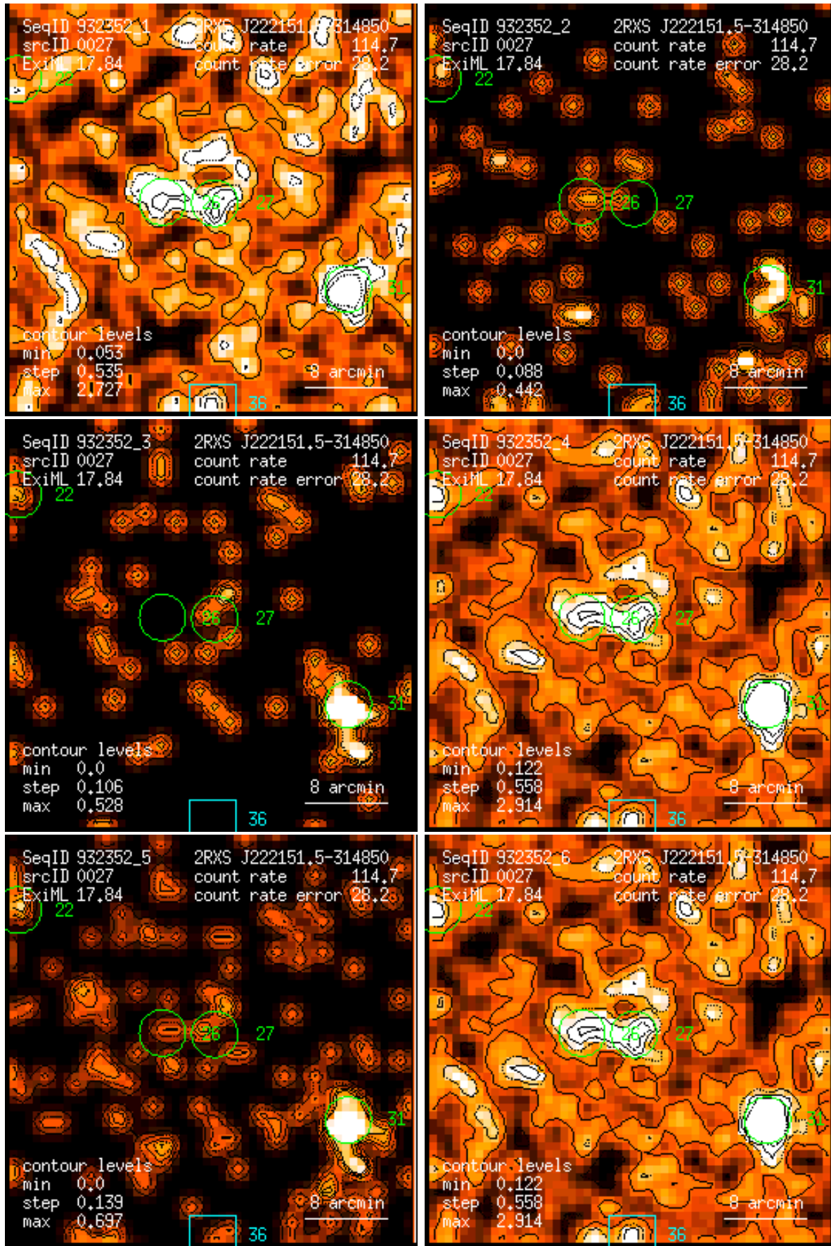
Figure 27: RASS 932352: detection 0027: band rate images, Gaussian filter: (1) PSPC channels 11 – 41, (2) 52 – 90, (3) 91 – 201, (4) 11 – 235, (5) 52 – 201, (6) 11 – 201. Broad band rates in counts/ks. Band rate contour levels in counts/ks/arcmin 2 .
