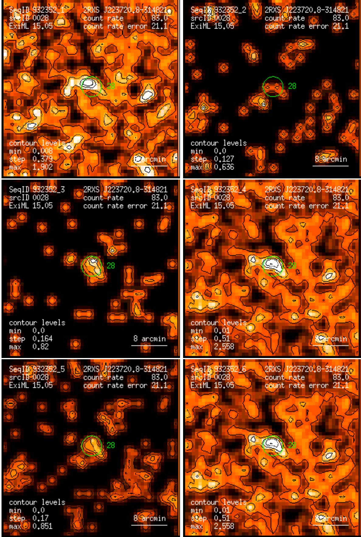
Figure 28: RASS 932352: detection 0028: band rate images, Gaussian filter: (1) PSPC channels 11 – 41, (2) 52 – 90, (3) 91 – 201, (4) 11 – 235, (5) 52 – 201, (6) 11 – 201. Broad band rates in counts/ks. Band rate contour levels in counts/ks/arcmin 2 .
