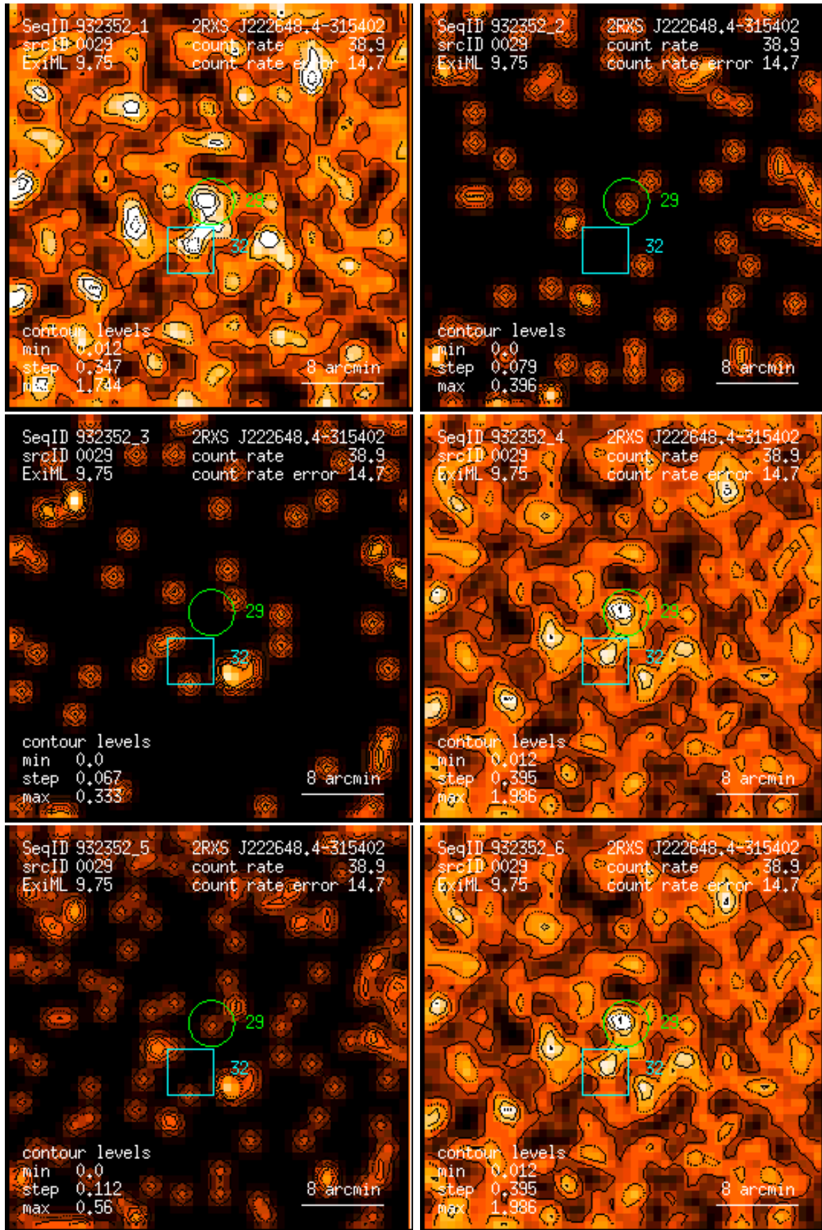
Figure 29: RASS 932352: detection 0029: band rate images, Gaussian filter: (1) PSPC channels 11 – 41, (2) 52 – 90, (3) 91 – 201, (4) 11 – 235, (5) 52 – 201, (6) 11 – 201. Broad band rates in counts/ks. Band rate contour levels in counts/ks/arcmin 2 .
