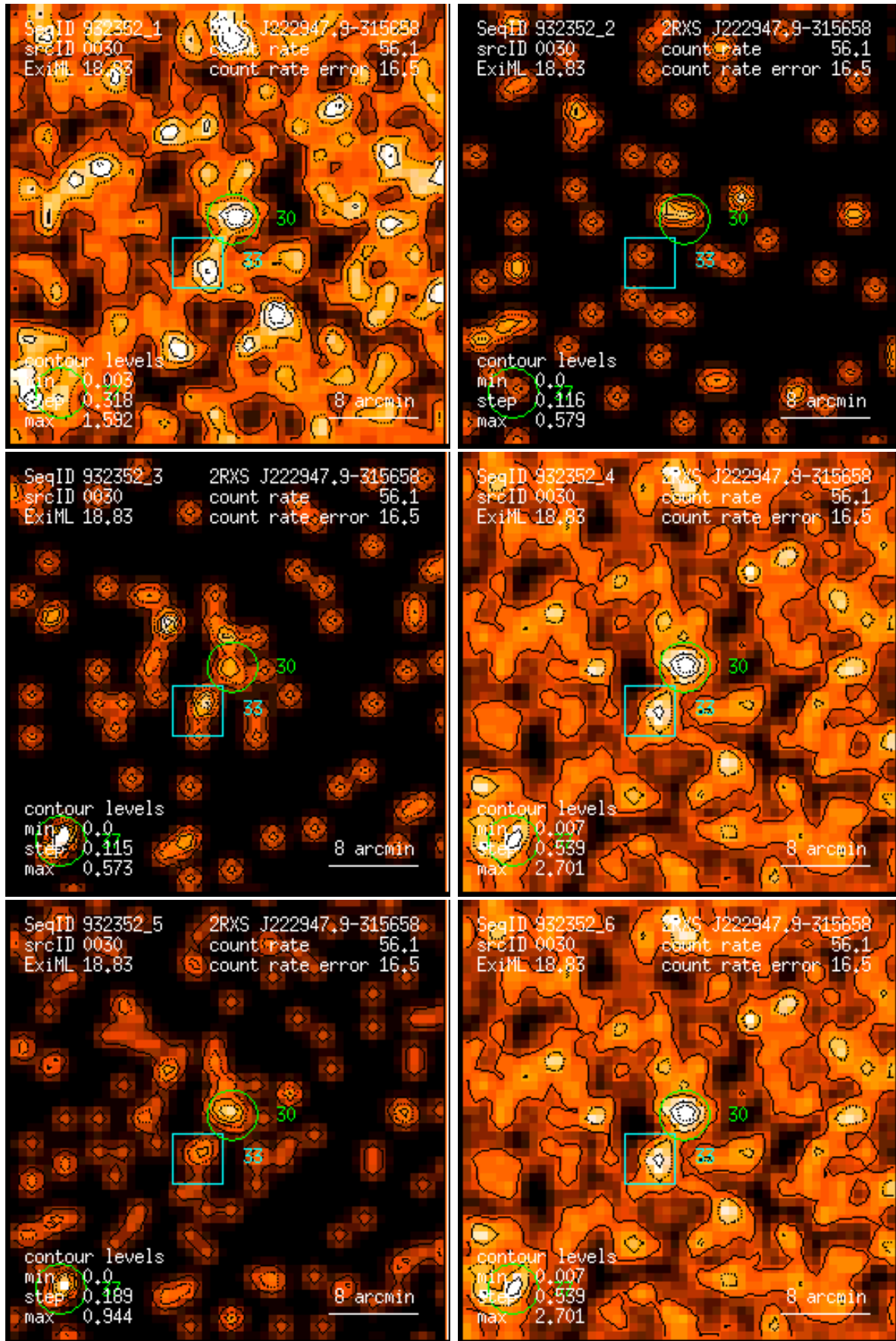
Figure 30: RASS 932352: detection 0030: band rate images, Gaussian filter: (1) PSPC channels 11 – 41, (2) 52 – 90, (3) 91 – 201, (4) 11 – 235, (5) 52 – 201, (6) 11 – 201. Broad band rates in counts/ks. Band rate contour levels in counts/ks/arcmin 2 .
