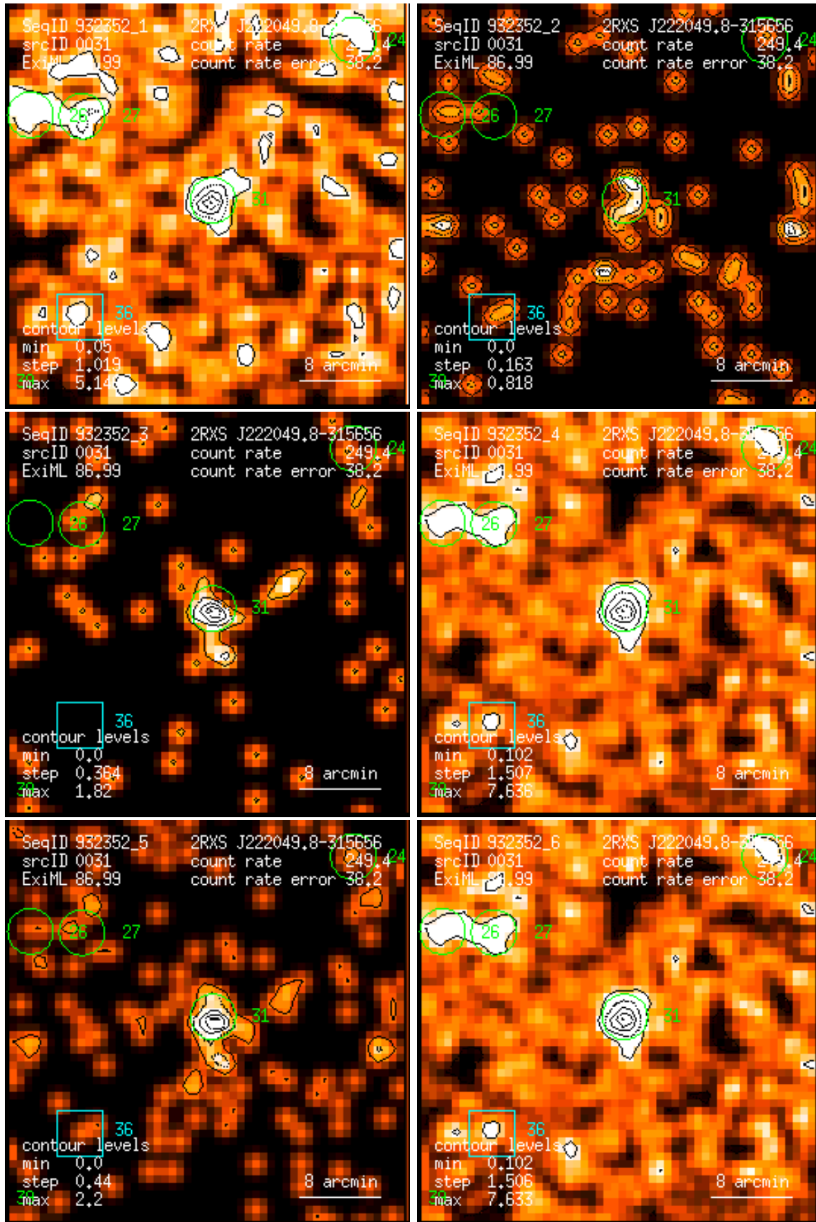
Figure 31: RASS 932352: detection 0031: band rate images, Gaussian filter: (1) PSPC channels 11 – 41, (2) 52 – 90, (3) 91 – 201, (4) 11 – 235, (5) 52 – 201, (6) 11 – 201. Broad band rates in counts/ks. Band rate contour levels in counts/ks/arcmin 2 .
