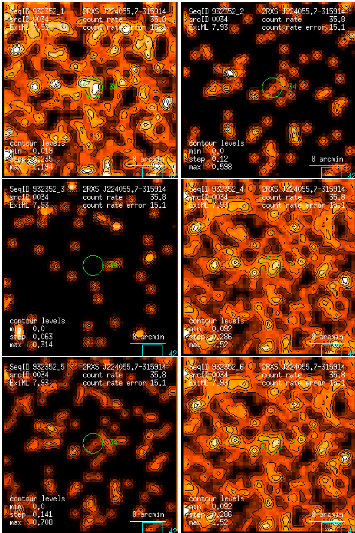
Figure 34: RASS 932352: detection 0034: band rate images, Gaussian filter: (1) PSPC channels 11 – 41, (2) 52 – 90, (3) 91 – 201, (4) 11 – 235, (5) 52 – 201, (6) 11 – 201. Broad band rates in counts/ks. Band rate contour levels in counts/ks/arcmin 2 .
