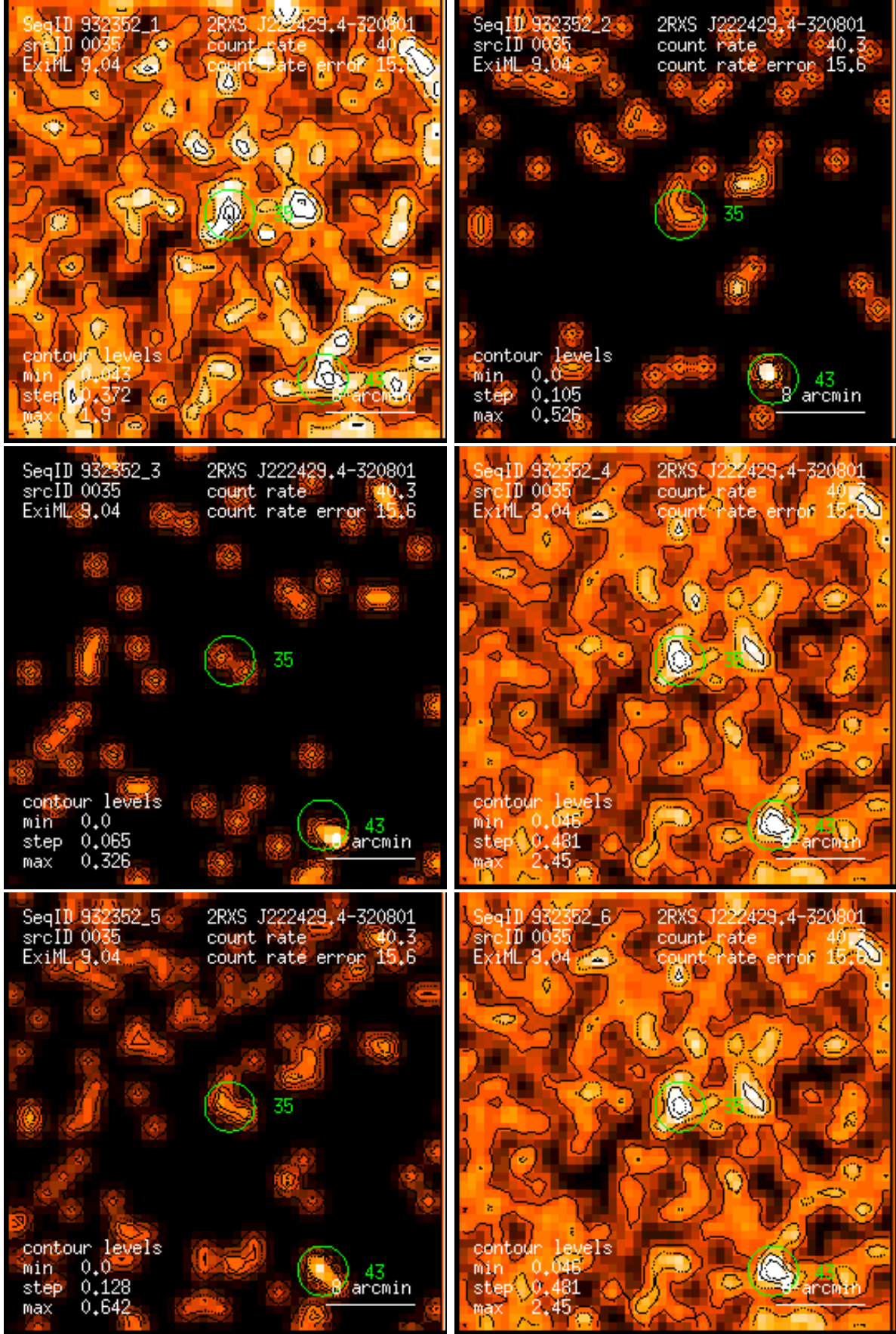
Figure 35: RASS 932352: detection 0035: band rate images, Gaussian filter: (1) PSPC channels 11 – 41, (2) 52 – 90, (3) 91 – 201, (4) 11 – 235, (5) 52 – 201, (6) 11 – 201. Broad band rates in counts/ks. Band rate contour levels in counts/ks/arcmin 2 .
