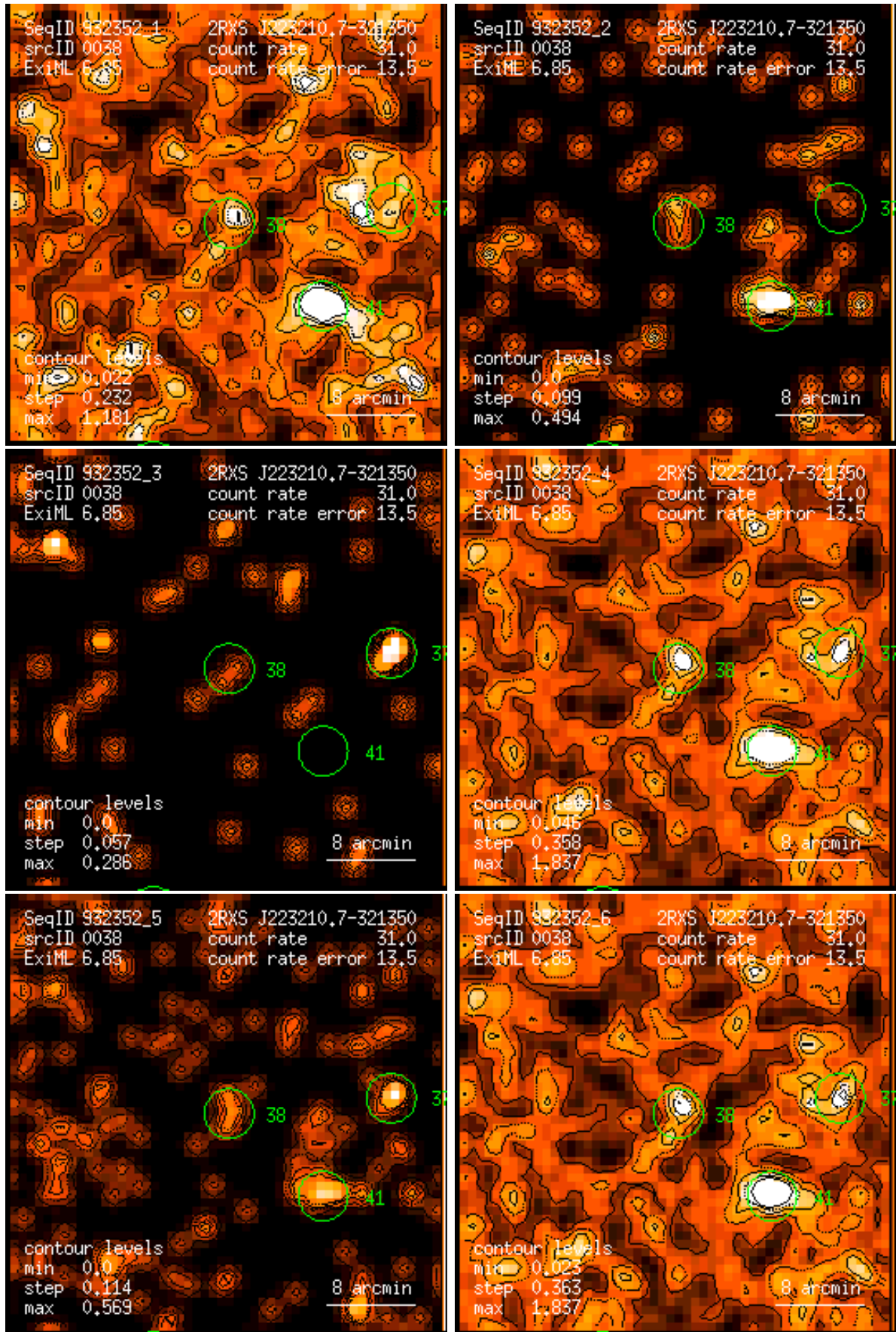
Figure 38: RASS 932352: detection 0038: band rate images, Gaussian filter: (1) PSPC channels 11 – 41, (2) 52 – 90, (3) 91 – 201, (4) 11 – 235, (5) 52 – 201, (6) 11 – 201. Broad band rates in counts/ks. Band rate contour levels in counts/ks/arcmin 2 .
