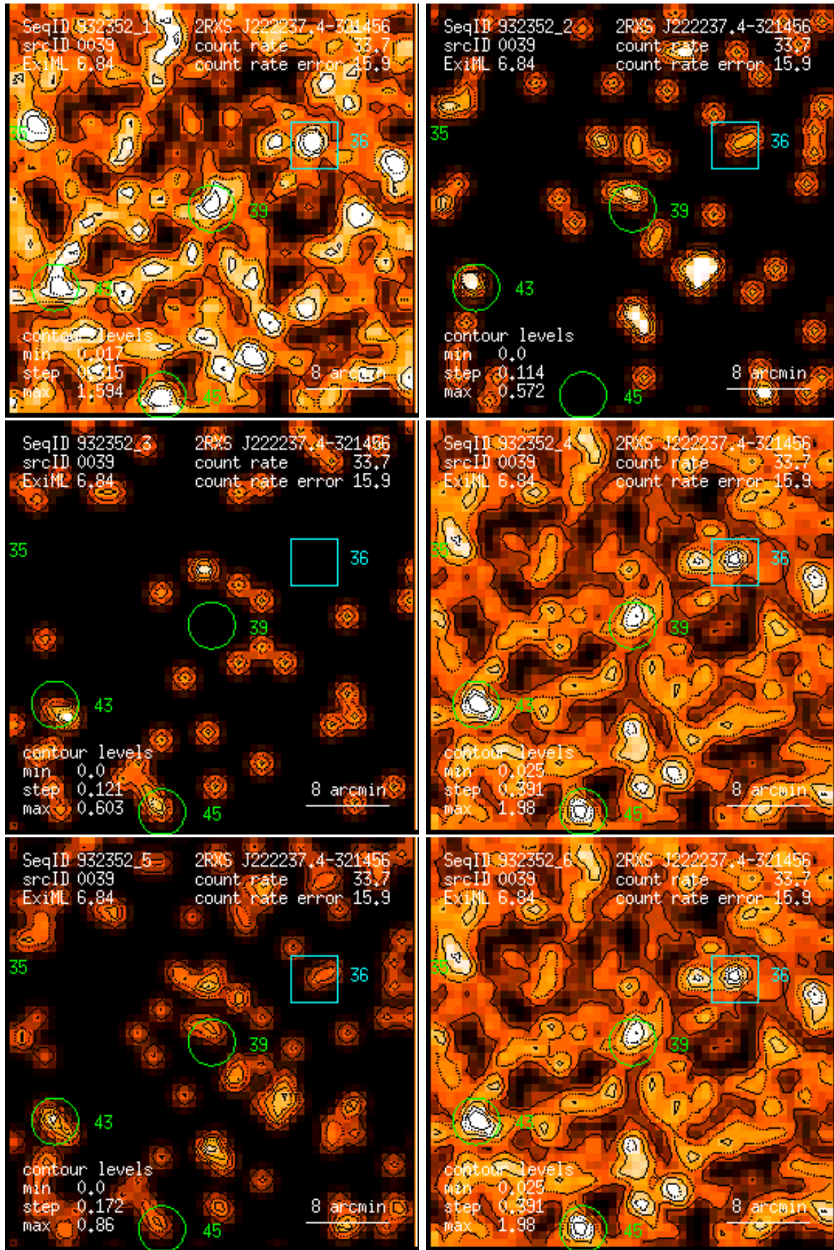
Figure 39: RASS 932352: detection 0039: band rate images, Gaussian filter: (1) PSPC channels 11 – 41, (2) 52 – 90, (3) 91 – 201, (4) 11 – 235, (5) 52 – 201, (6) 11 – 201. Broad band rates in counts/ks. Band rate contour levels in counts/ks/arcmin 2 .
