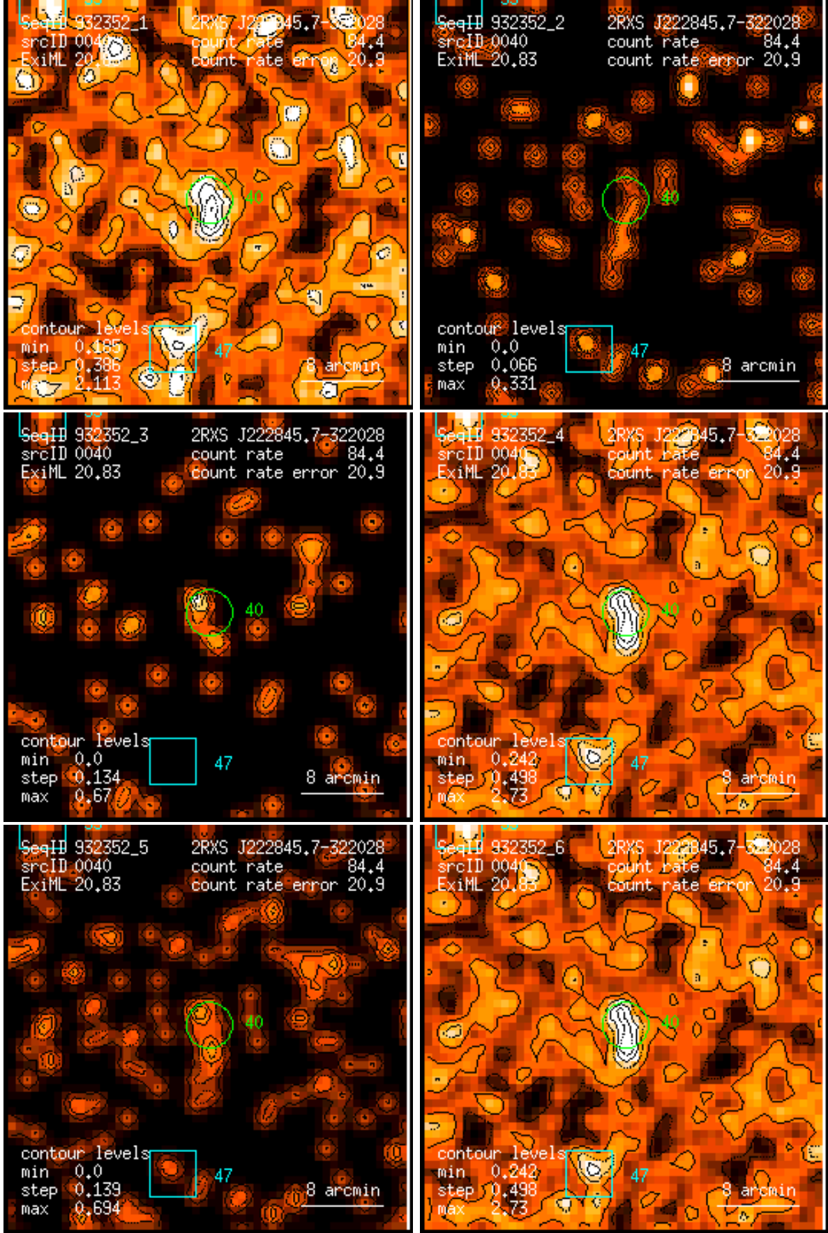
Figure 40: RASS 932352: detection 0040: band rate images, Gaussian filter: (1) PSPC channels 11 – 41, (2) 52 – 90, (3) 91 – 201, (4) 11 – 235, (5) 52 – 201, (6) 11 – 201. Broad band rates in counts/ks. Band rate contour levels in counts/ks/arcmin 2 .
