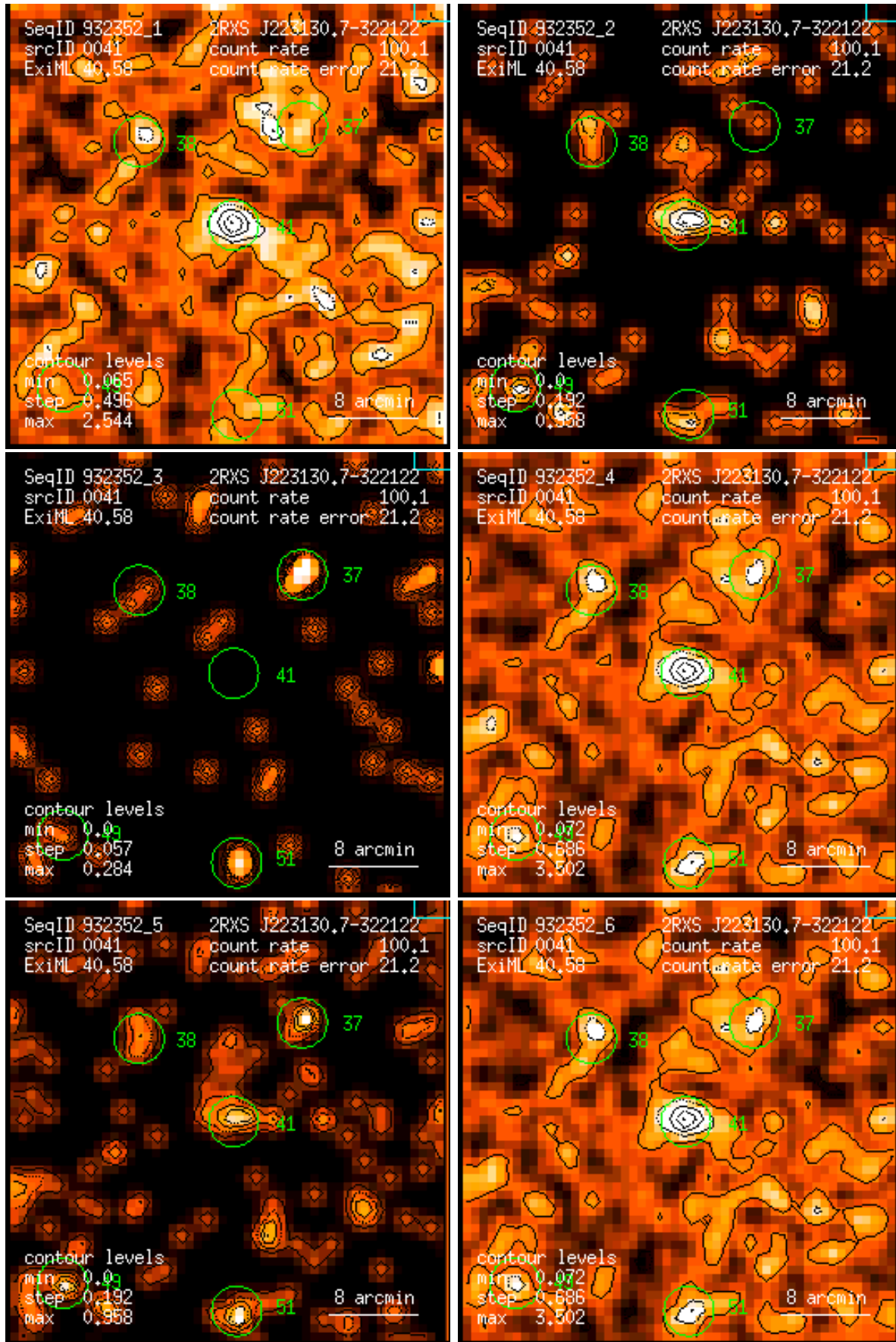
Figure 41: RASS 932352: detection 0041: band rate images, Gaussian filter: (1) PSPC channels 11 – 41, (2) 52 – 90, (3) 91 – 201, (4) 11 – 235, (5) 52 – 201, (6) 11 – 201. Broad band rates in counts/ks. Band rate contour levels in counts/ks/arcmin 2 .
