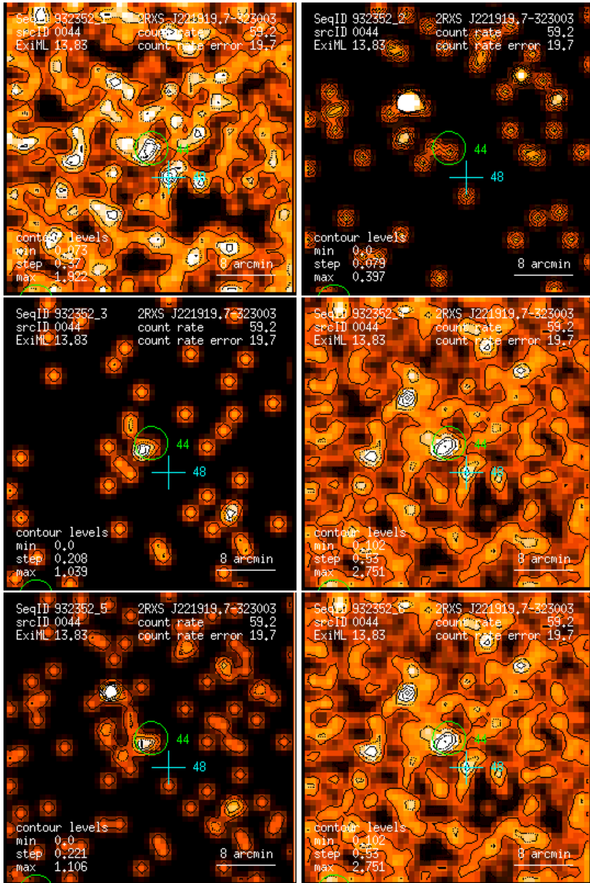
Figure 44: RASS 932352: detection 0044: band rate images, Gaussian filter: (1) PSPC channels 11 – 41, (2) 52 – 90, (3) 91 – 201, (4) 11 – 235, (5) 52 – 201, (6) 11 – 201. Broad band rates in counts/ks. Band rate contour levels in counts/ks/arcmin 2 .
