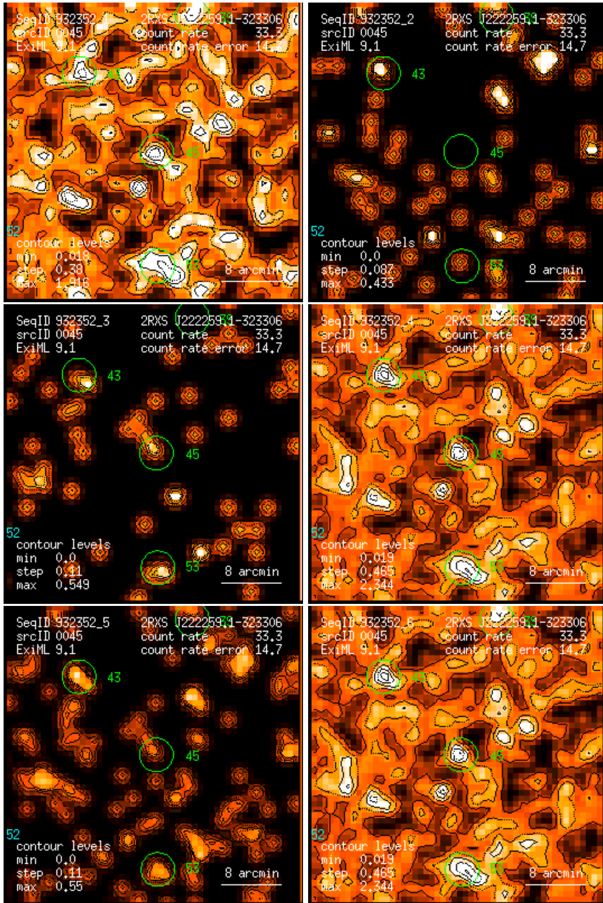
Figure 45: RASS 932352: detection 0045: band rate images, Gaussian filter: (1) PSPC channels 11 – 41, (2) 52 – 90, (3) 91 – 201, (4) 11 – 235, (5) 52 – 201, (6) 11 – 201. Broad band rates in counts/ks. Band rate contour levels in counts/ks/arcmin 2 .
