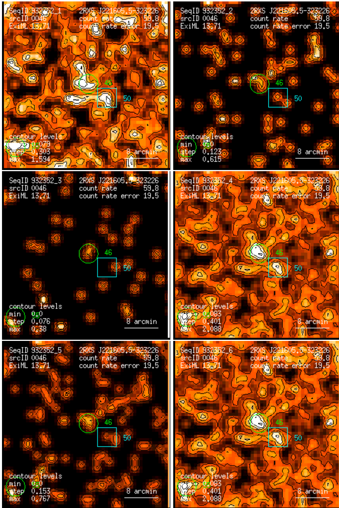
Figure 46: RASS 932352: detection 0046: band rate images, Gaussian filter: (1) PSPC channels 11 – 41, (2) 52 – 90, (3) 91 – 201, (4) 11 – 235, (5) 52 – 201, (6) 11 – 201. Broad band rates in counts/ks. Band rate contour levels in counts/ks/arcmin 2 .
