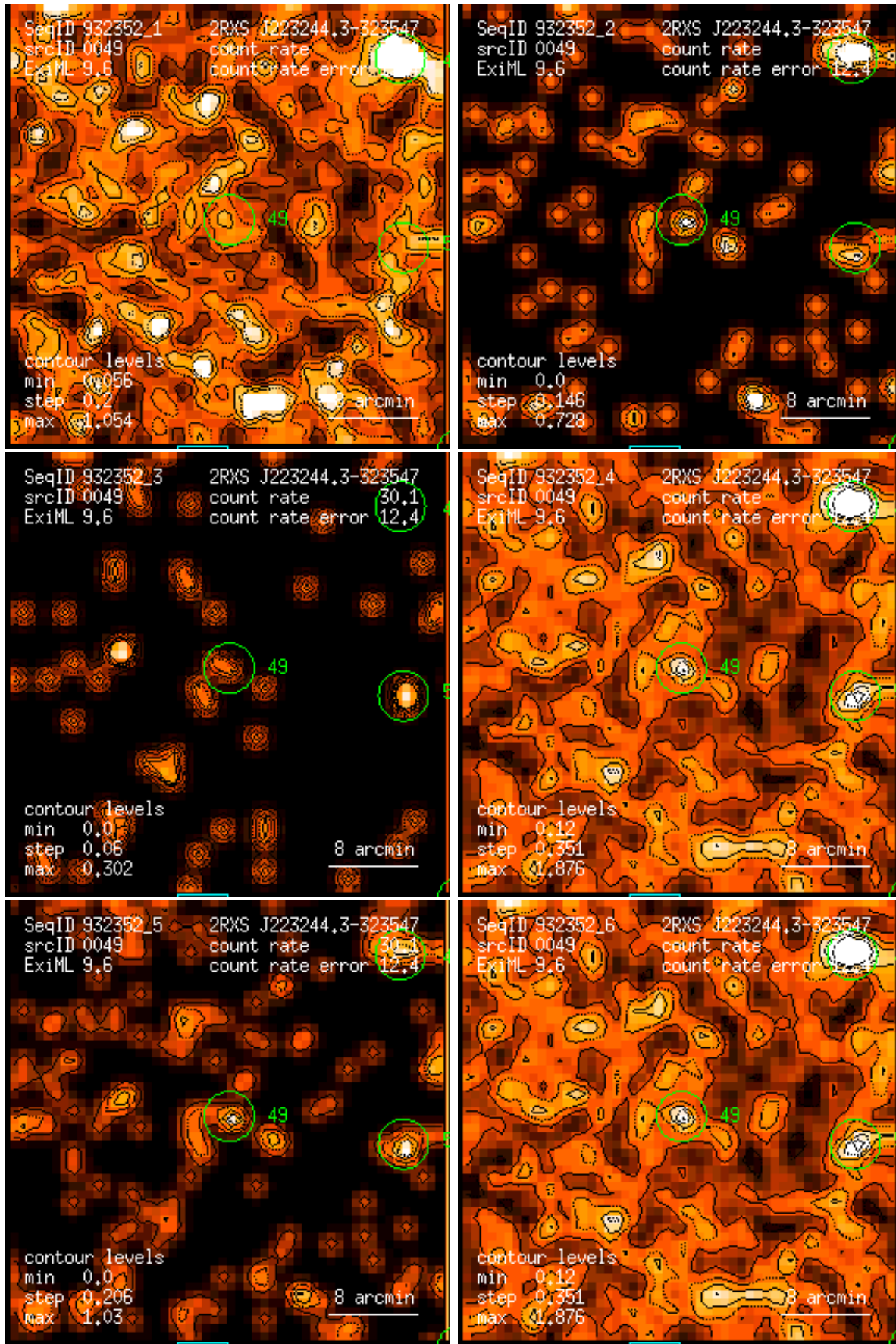
Figure 49: RASS 932352: detection 0049: band rate images, Gaussian filter: (1) PSPC channels 11 – 41, (2) 52 – 90, (3) 91 – 201, (4) 11 – 235, (5) 52 – 201, (6) 11 – 201. Broad band rates in counts/ks. Band rate contour levels in counts/ks/arcmin 2 .
