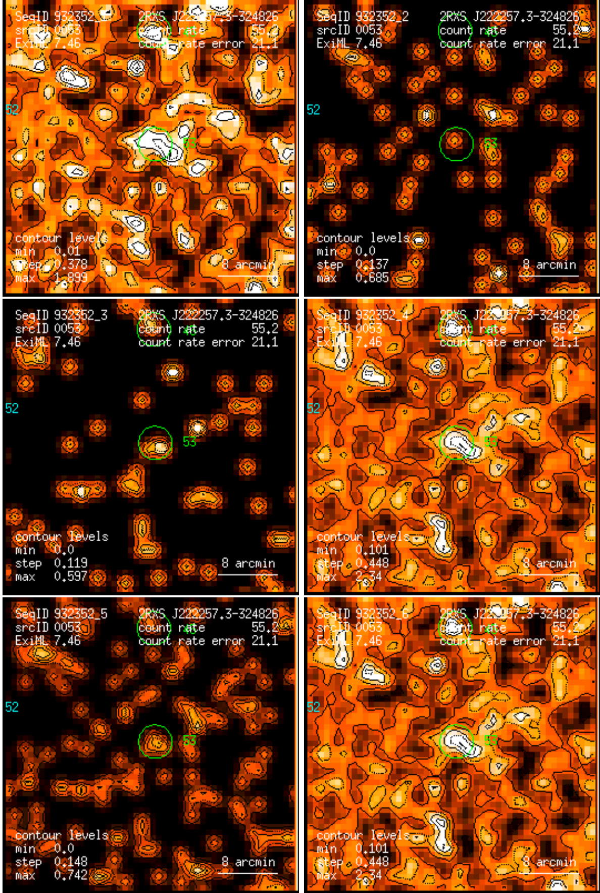
Figure 53: RASS 932352: detection 0053: band rate images, Gaussian filter: (1) PSPC channels 11 – 41, (2) 52 – 90, (3) 91 – 201, (4) 11 – 235, (5) 52 – 201, (6) 11 – 201. Broad band rates in counts/ks. Band rate contour levels in counts/ks/arcmin 2 .
