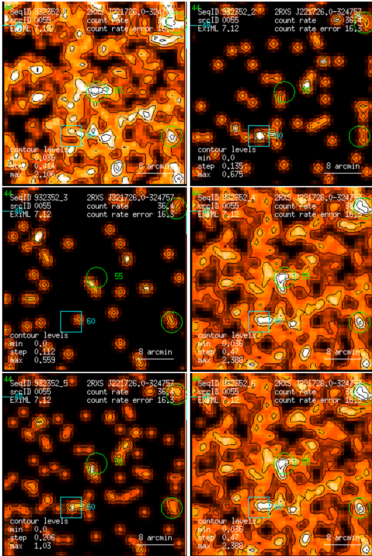
Figure 55: RASS 932352: detection 0055: band rate images, Gaussian filter: (1) PSPC channels 11 – 41, (2) 52 – 90, (3) 91 – 201, (4) 11 – 235, (5) 52 – 201, (6) 11 – 201. Broad band rates in counts/ks. Band rate contour levels in counts/ks/arcmin 2 .
