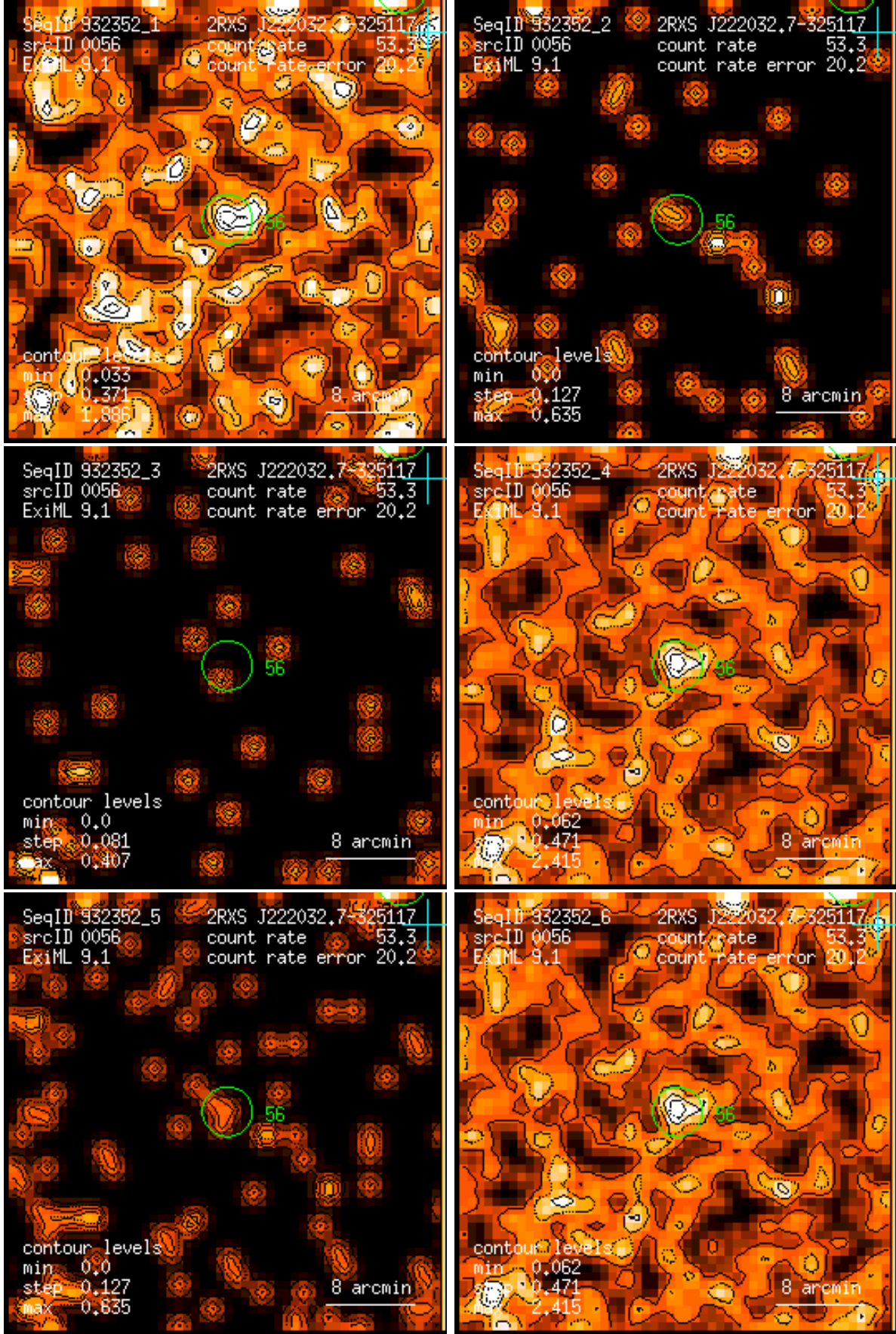
Figure 56: RASS 932352: detection 0056: band rate images, Gaussian filter: (1) PSPC channels 11 – 41, (2) 52 – 90, (3) 91 – 201, (4) 11 – 235, (5) 52 – 201, (6) 11 – 201. Broad band rates in counts/ks. Band rate contour levels in counts/ks/arcmin 2 .
