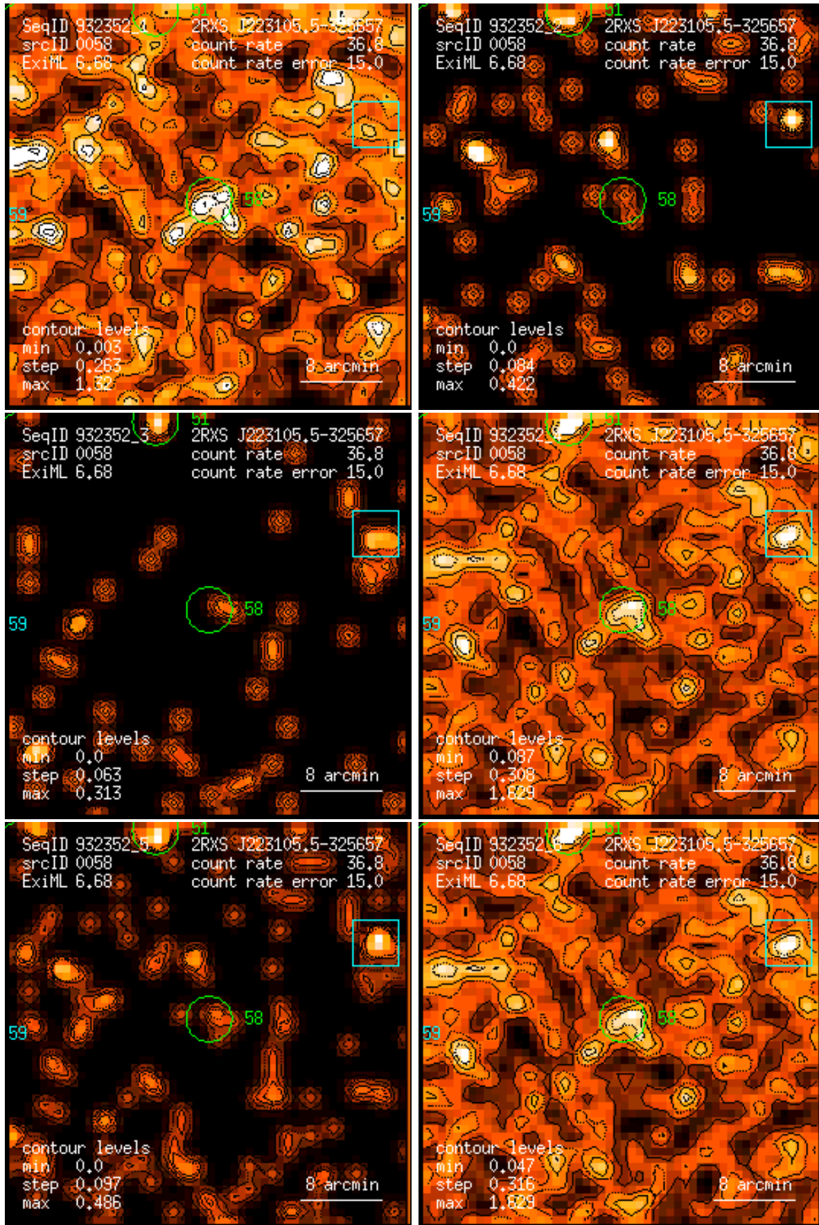
Figure 58: RASS 932352: detection 0058: band rate images, Gaussian filter: (1) PSPC channels 11 – 41, (2) 52 – 90, (3) 91 – 201, (4) 11 – 235, (5) 52 – 201, (6) 11 – 201. Broad band rates in counts/ks. Band rate contour levels in counts/ks/arcmin 2 .
