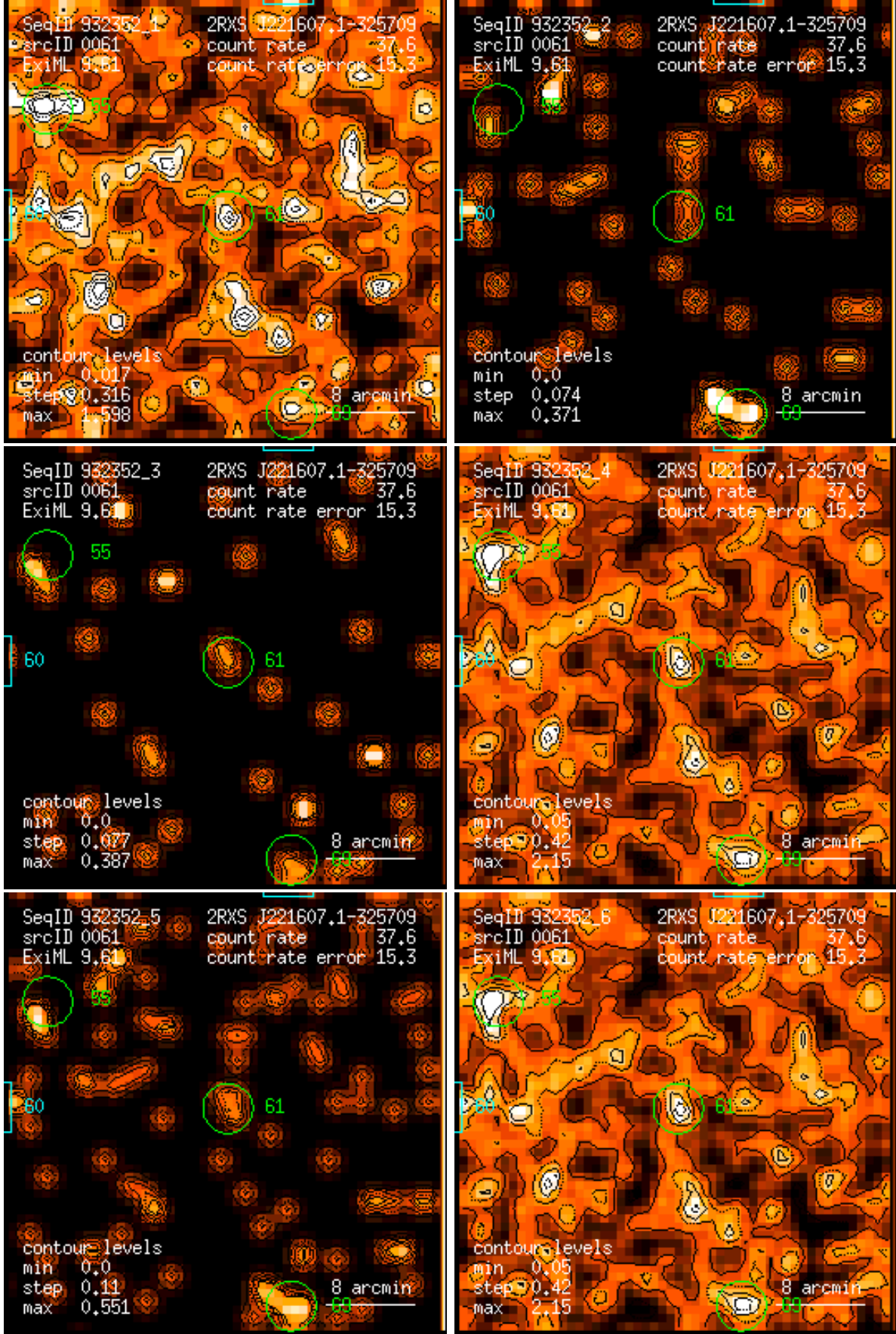
Figure 61: RASS 932352: detection 0061: band rate images, Gaussian filter: (1) PSPC channels 11 – 41, (2) 52 – 90, (3) 91 – 201, (4) 11 – 235, (5) 52 – 201, (6) 11 – 201. Broad band rates in counts/ks. Band rate contour levels in counts/ks/arcmin 2 .
