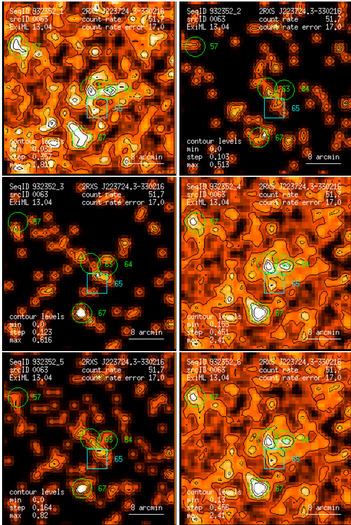
Figure 63: RASS 932352: detection 0063: band rate images, Gaussian filter: (1) PSPC channels 11 – 41, (2) 52 – 90, (3) 91 – 201, (4) 11 – 235, (5) 52 – 201, (6) 11 – 201. Broad band rates in counts/ks. Band rate contour levels in counts/ks/arcmin 2 .
