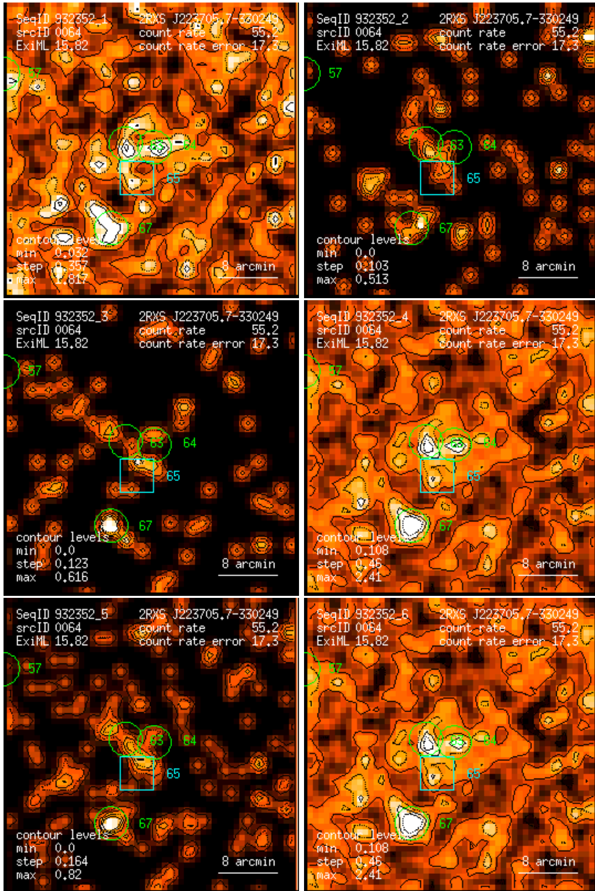
Figure 64: RASS 932352: detection 0064: band rate images, Gaussian filter: (1) PSPC channels 11 – 41, (2) 52 – 90, (3) 91 – 201, (4) 11 – 235, (5) 52 – 201, (6) 11 – 201. Broad band rates in counts/ks. Band rate contour levels in counts/ks/arcmin 2 .
