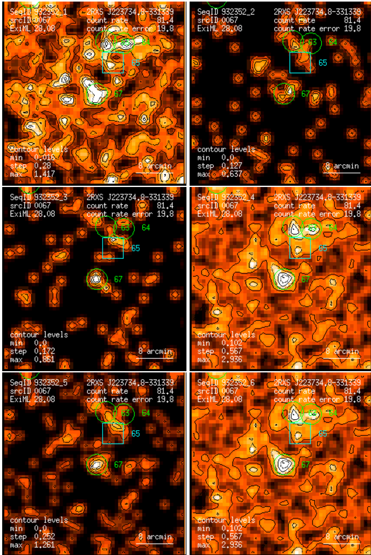
Figure 67: RASS 932352: detection 0067: band rate images, Gaussian filter: (1) PSPC channels 11 – 41, (2) 52 – 90, (3) 91 – 201, (4) 11 – 235, (5) 52 – 201, (6) 11 – 201. Broad band rates in counts/ks. Band rate contour levels in counts/ks/arcmin 2 .
