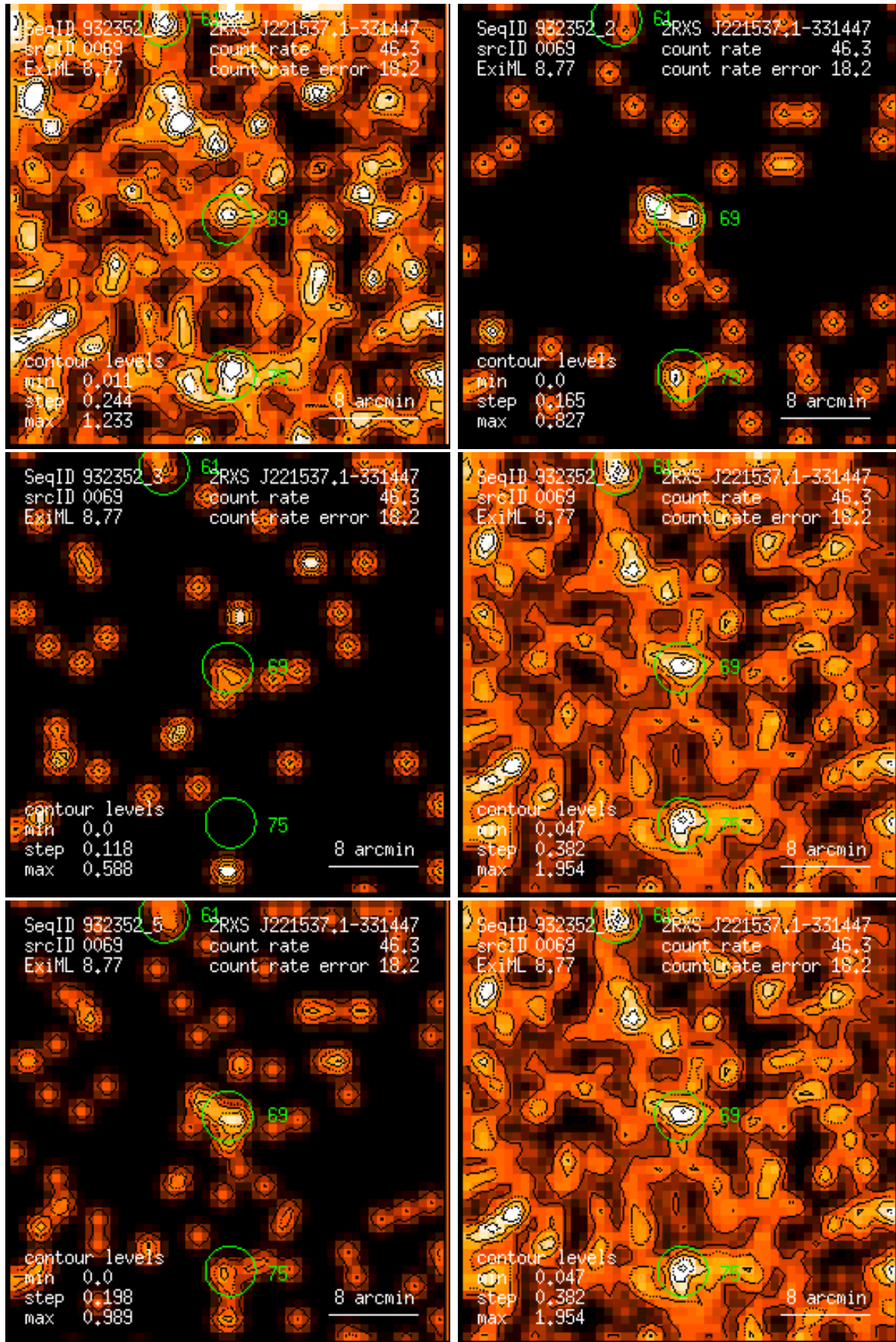
Figure 69: RASS 932352: detection 0069: band rate images, Gaussian filter: (1) PSPC channels 11 – 41, (2) 52 – 90, (3) 91 – 201, (4) 11 – 235, (5) 52 – 201, (6) 11 – 201. Broad band rates in counts/ks. Band rate contour levels in counts/ks/arcmin 2 .
