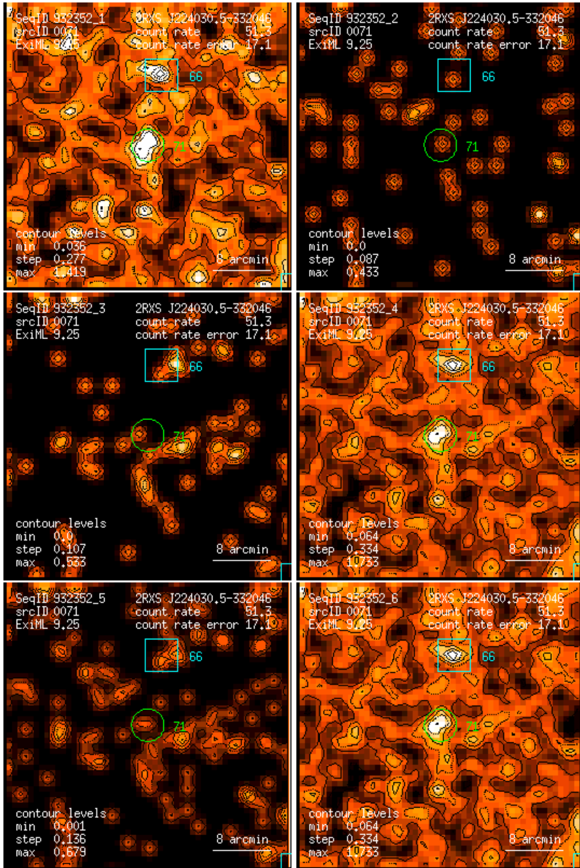
Figure 71: RASS 932352: detection 0071: band rate images, Gaussian filter: (1) PSPC channels 11 – 41, (2) 52 – 90, (3) 91 – 201, (4) 11 – 235, (5) 52 – 201, (6) 11 – 201. Broad band rates in counts/ks. Band rate contour levels in counts/ks/arcmin 2 .
