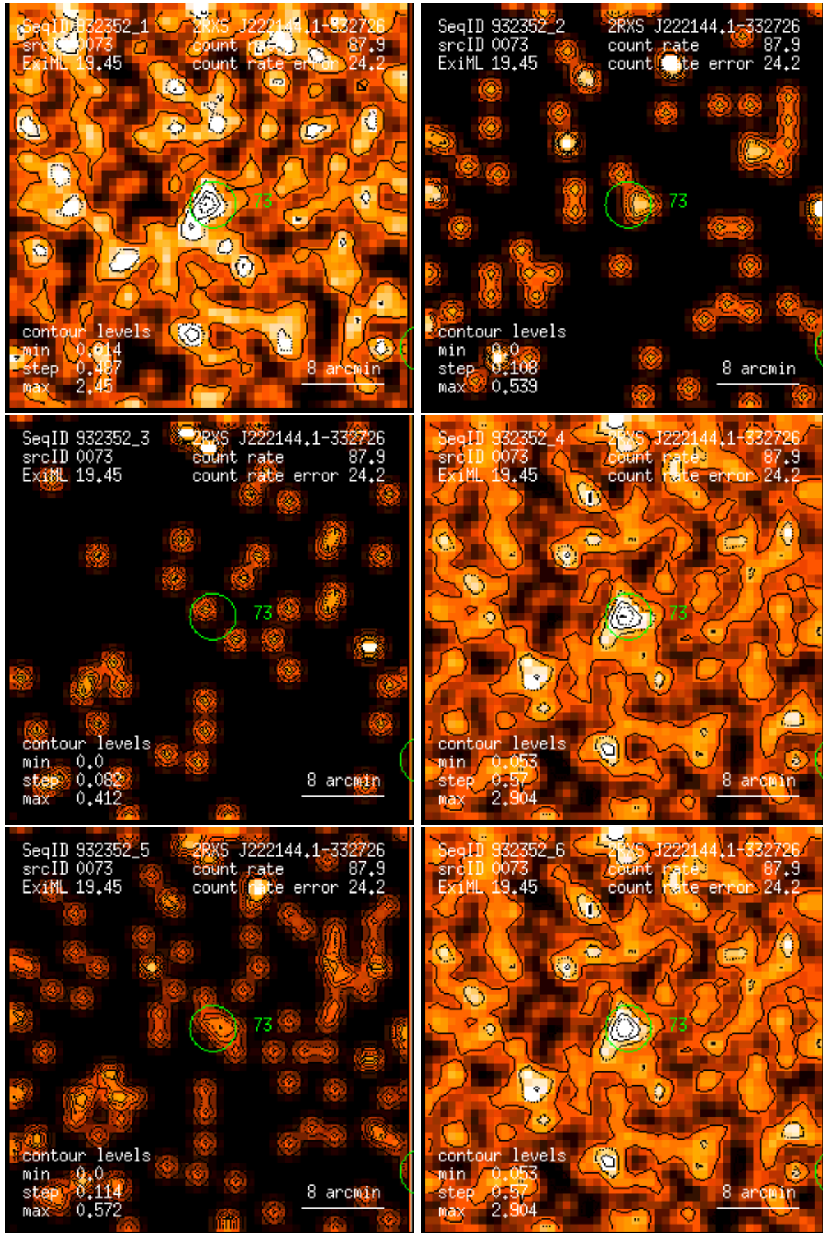
Figure 73: RASS 932352: detection 0073: band rate images, Gaussian filter: (1) PSPC channels 11 – 41, (2) 52 – 90, (3) 91 – 201, (4) 11 – 235, (5) 52 – 201, (6) 11 – 201. Broad band rates in counts/ks. Band rate contour levels in counts/ks/arcmin 2 .
