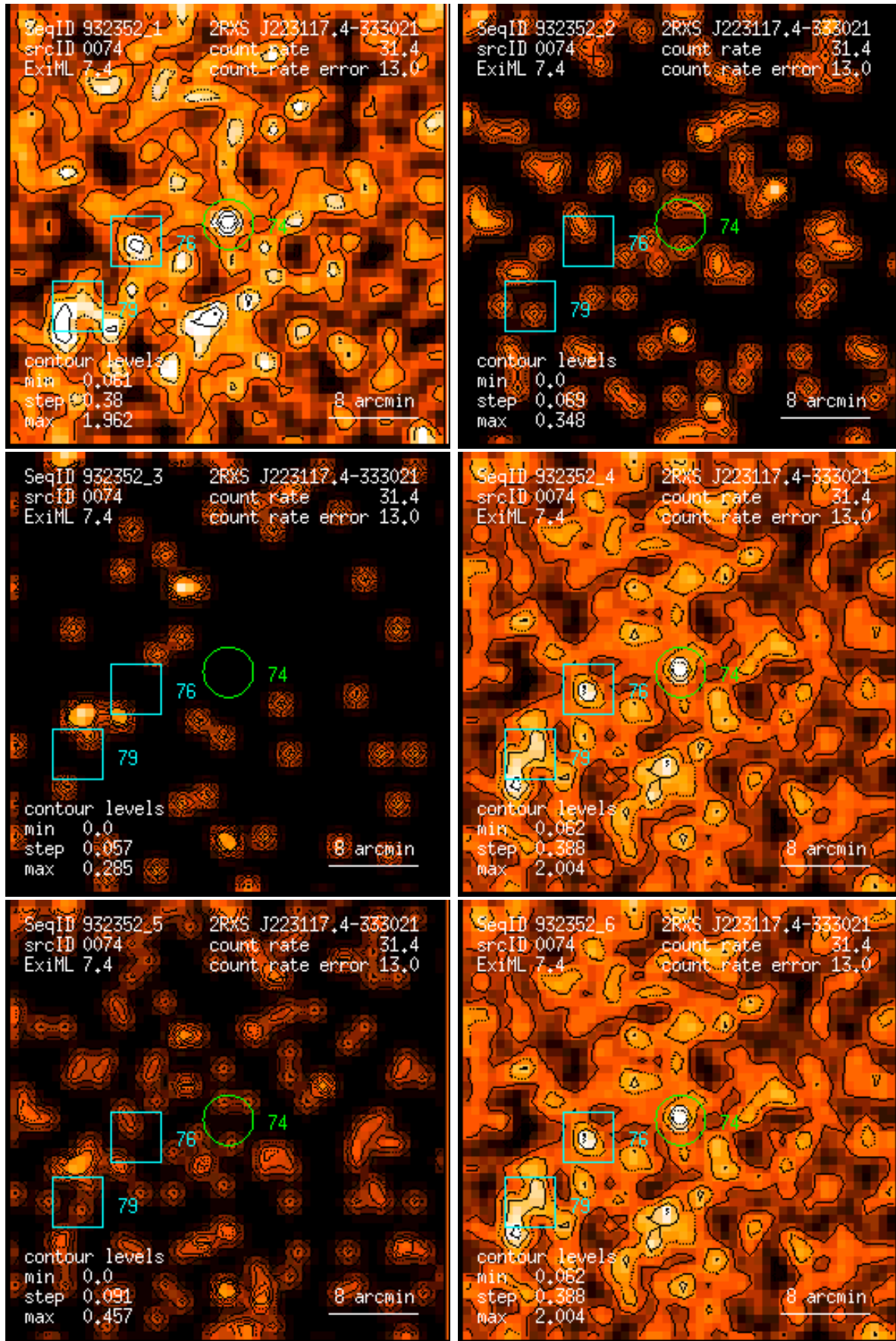
Figure 74: RASS 932352: detection 0074: band rate images, Gaussian filter: (1) PSPC channels 11 – 41, (2) 52 – 90, (3) 91 – 201, (4) 11 – 235, (5) 52 – 201, (6) 11 – 201. Broad band rates in counts/ks. Band rate contour levels in counts/ks/arcmin 2 .
