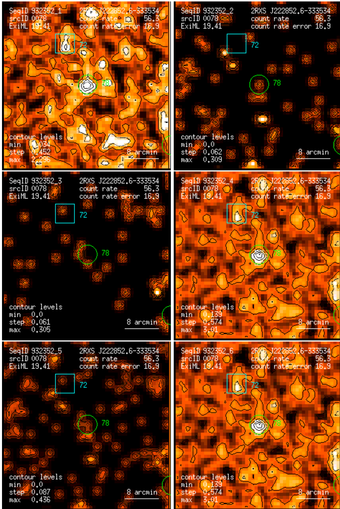
Figure 78: RASS 932352: detection 0078: band rate images, Gaussian filter: (1) PSPC channels 11 – 41, (2) 52 – 90, (3) 91 – 201, (4) 11 – 235, (5) 52 – 201, (6) 11 – 201. Broad band rates in counts/ks. Band rate contour levels in counts/ks/arcmin 2 .
