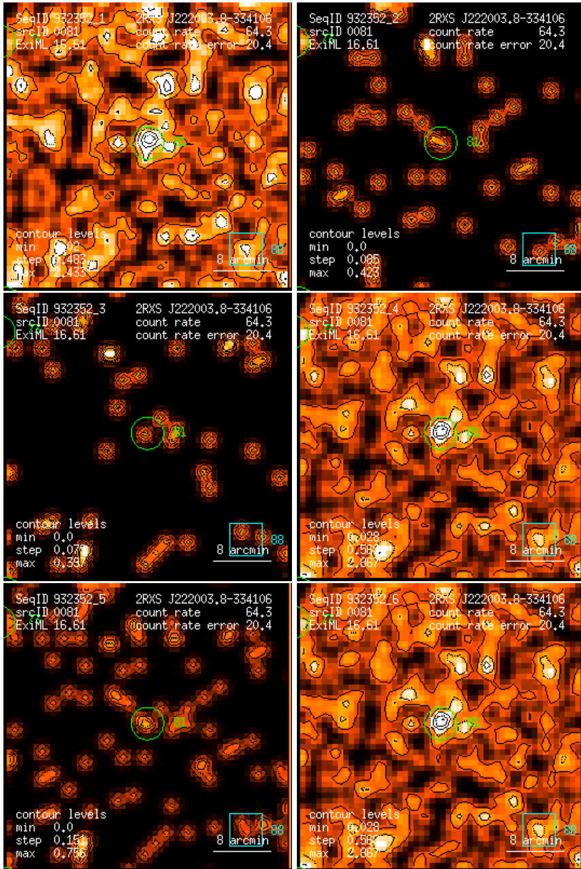
Figure 81: RASS 932352: detection 0081: band rate images, Gaussian filter: (1) PSPC channels 11 – 41, (2) 52 – 90, (3) 91 – 201, (4) 11 – 235, (5) 52 – 201, (6) 11 – 201. Broad band rates in counts/ks. Band rate contour levels in counts/ks/arcmin 2 .
