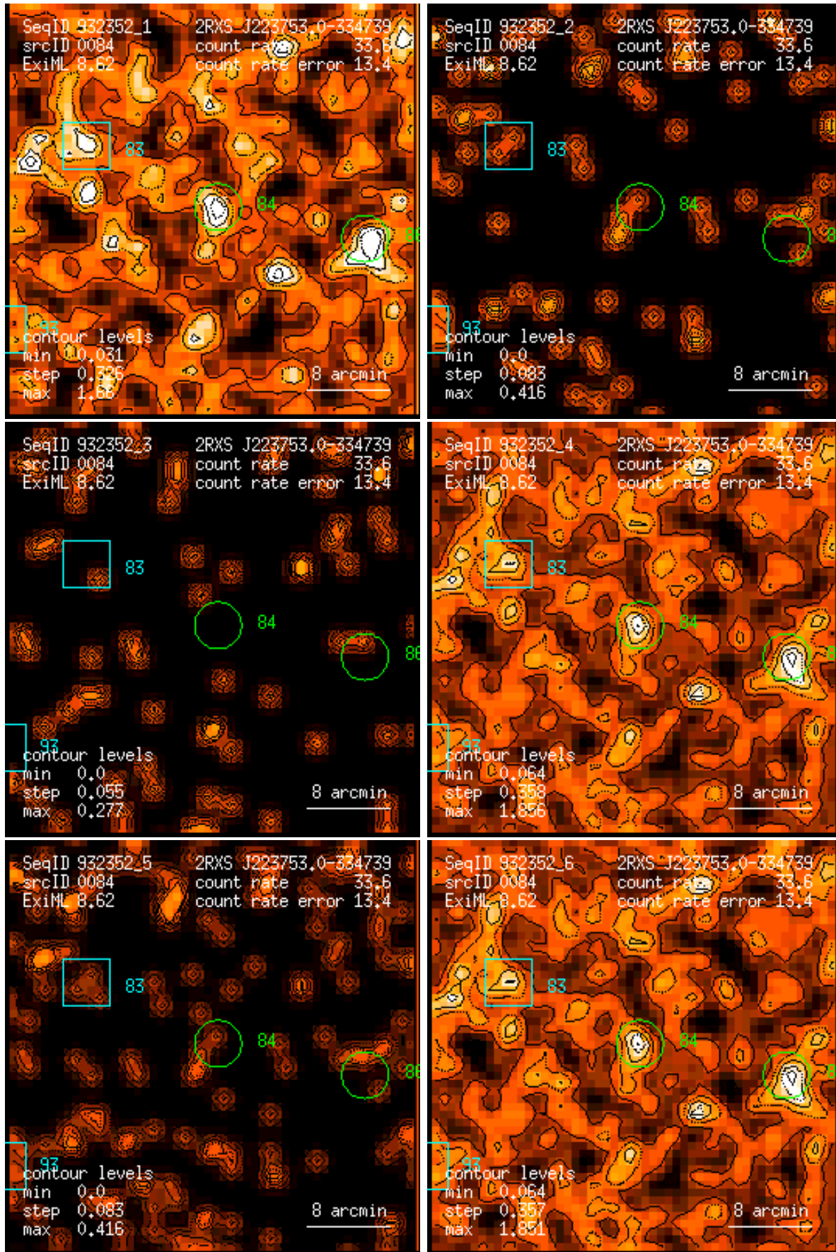
Figure 84: RASS 932352: detection 0084: band rate images, Gaussian filter: (1) PSPC channels 11 – 41, (2) 52 – 90, (3) 91 – 201, (4) 11 – 235, (5) 52 – 201, (6) 11 – 201. Broad band rates in counts/ks. Band rate contour levels in counts/ks/arcmin 2 .
