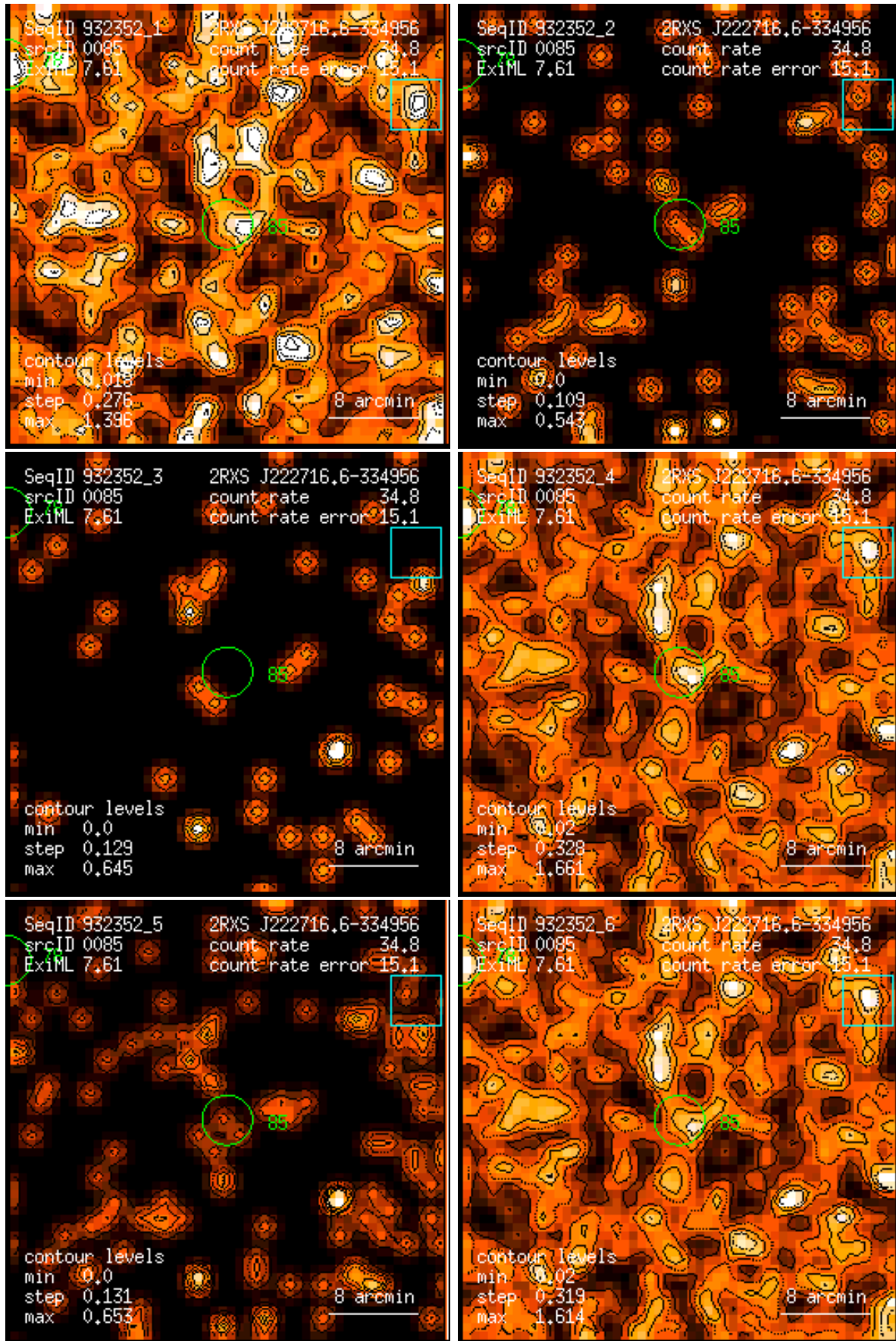
Figure 85: RASS 932352: detection 0085: band rate images, Gaussian filter: (1) PSPC channels 11 – 41, (2) 52 – 90, (3) 91 – 201, (4) 11 – 235, (5) 52 – 201, (6) 11 – 201. Broad band rates in counts/ks. Band rate contour levels in counts/ks/arcmin 2 .
