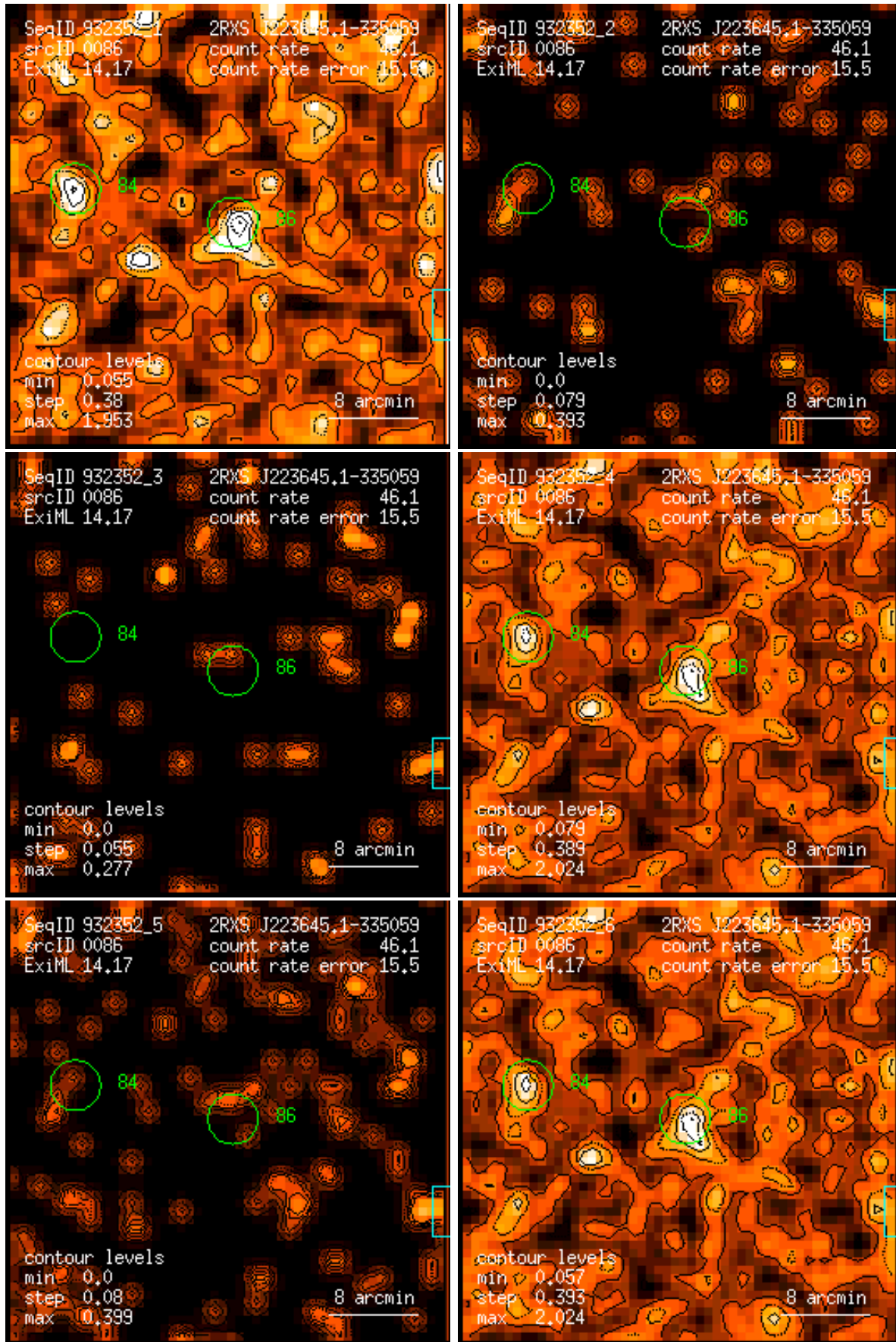
Figure 86: RASS 932352: detection 0086: band rate images, Gaussian filter: (1) PSPC channels 11 – 41, (2) 52 – 90, (3) 91 – 201, (4) 11 – 235, (5) 52 – 201, (6) 11 – 201. Broad band rates in counts/ks. Band rate contour levels in counts/ks/arcmin 2 .
