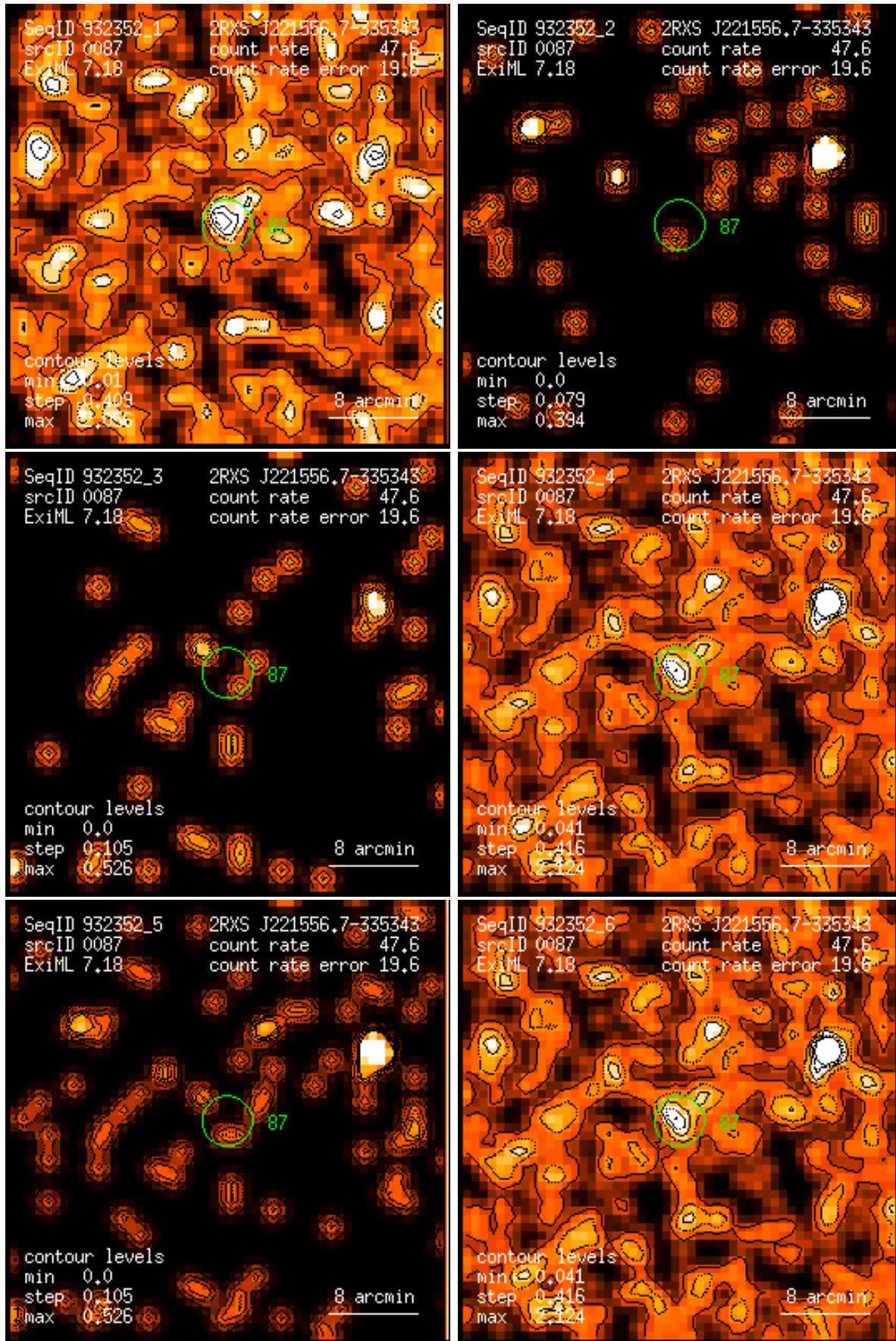
Figure 87: RASS 932352: detection 0087: band rate images, Gaussian filter: (1) PSPC channels 11 – 41, (2) 52 – 90, (3) 91 – 201, (4) 11 – 235, (5) 52 – 201, (6) 11 – 201. Broad band rates in counts/ks. Band rate contour levels in counts/ks/arcmin 2 .
