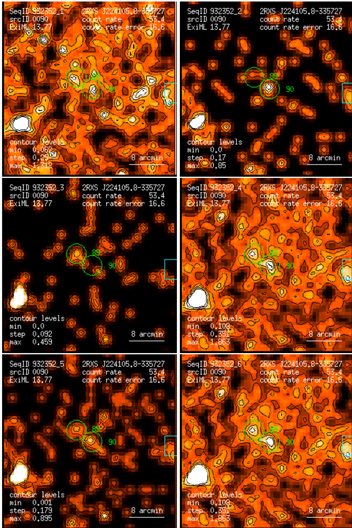
Figure 90: RASS 932352: detection 0090: band rate images, Gaussian filter: (1) PSPC channels 11 – 41, (2) 52 – 90, (3) 91 – 201, (4) 11 – 235, (5) 52 – 201, (6) 11 – 201. Broad band rates in counts/ks. Band rate contour levels in counts/ks/arcmin 2 .
