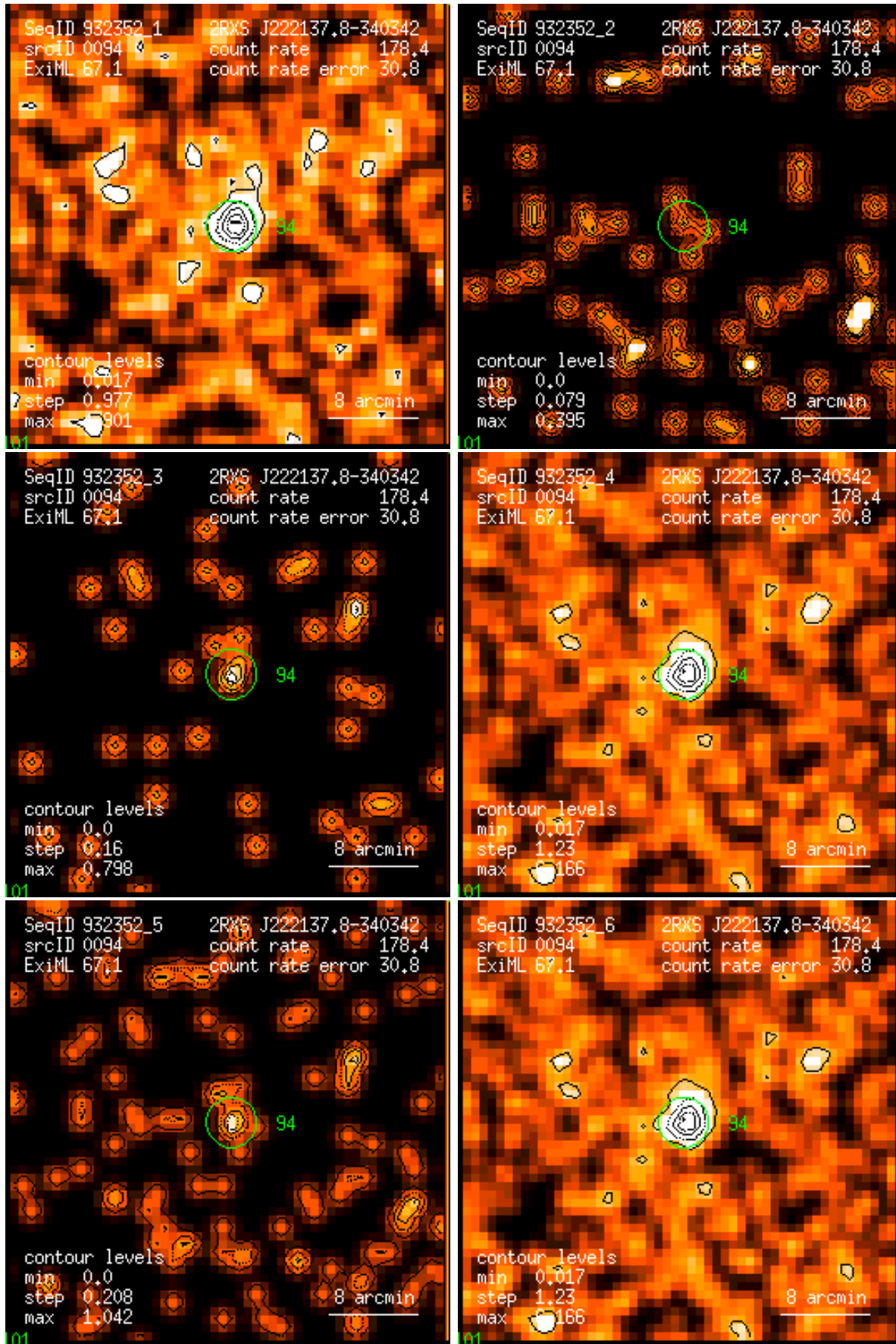
Figure 94: RASS 932352: detection 0094: band rate images, Gaussian filter: (1) PSPC channels 11 – 41, (2) 52 – 90, (3) 91 – 201, (4) 11 – 235, (5) 52 – 201, (6) 11 – 201. Broad band rates in counts/ks. Band rate contour levels in counts/ks/arcmin 2 .
