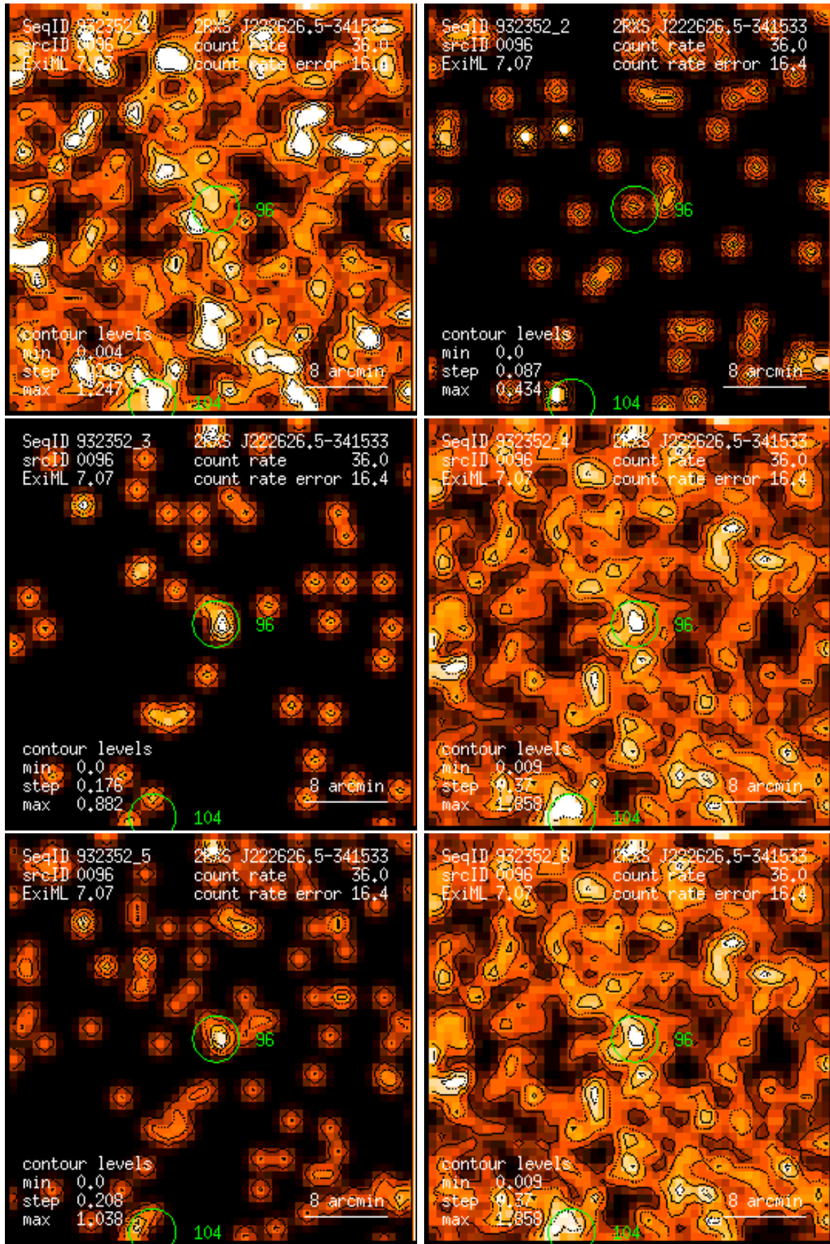
Figure 96: RASS 932352: detection 0096: band rate images, Gaussian filter: (1) PSPC channels 11 – 41, (2) 52 – 90, (3) 91 – 201, (4) 11 – 235, (5) 52 – 201, (6) 11 – 201. Broad band rates in counts/ks. Band rate contour levels in counts/ks/arcmin 2 .
