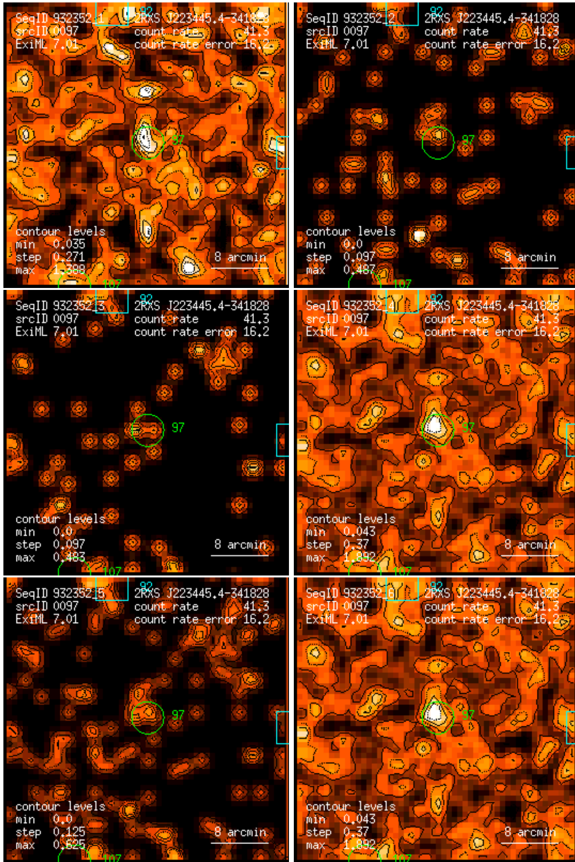
Figure 97: RASS 932352: detection 0097: band rate images, Gaussian filter: (1) PSPC channels 11 – 41, (2) 52 – 90, (3) 91 – 201, (4) 11 – 235, (5) 52 – 201, (6) 11 – 201. Broad band rates in counts/ks. Band rate contour levels in counts/ks/arcmin 2 .
