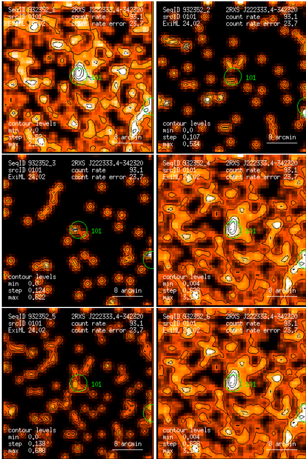
Figure 101: RASS 932352: detection 0101: band rate images, Gaussian filter: (1) PSPC channels 11 – 41, (2) 52 – 90, (3) 91 – 201, (4) 11 – 235, (5) 52 – 201, (6) 11 – 201. Broad band rates in counts/ks. Band rate contour levels in counts/ks/arcmin 2 .
