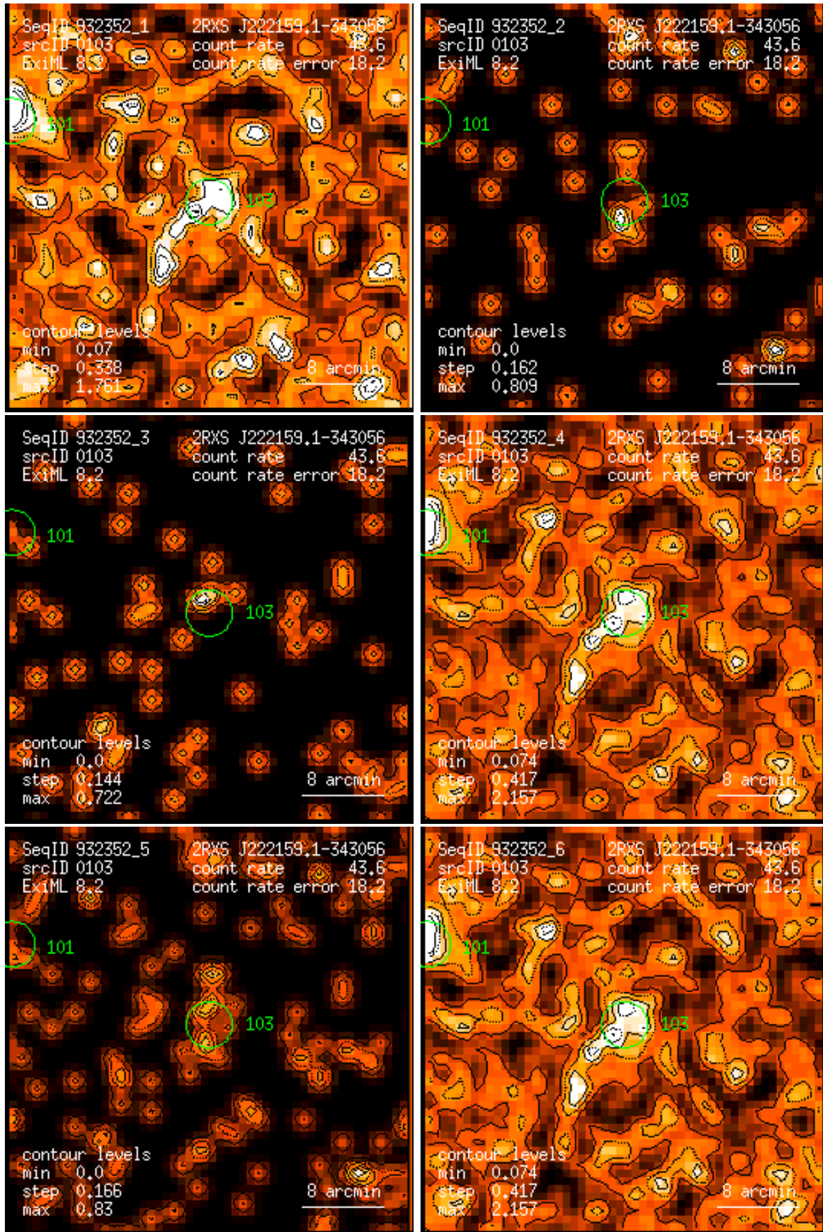
Figure 103: RASS 932352: detection 0103: band rate images, Gaussian filter: (1) PSPC channels 11 – 41, (2) 52 – 90, (3) 91 – 201, (4) 11 – 235, (5) 52 – 201, (6) 11 – 201. Broad band rates in counts/ks. Band rate contour levels in counts/ks/arcmin 2 .
