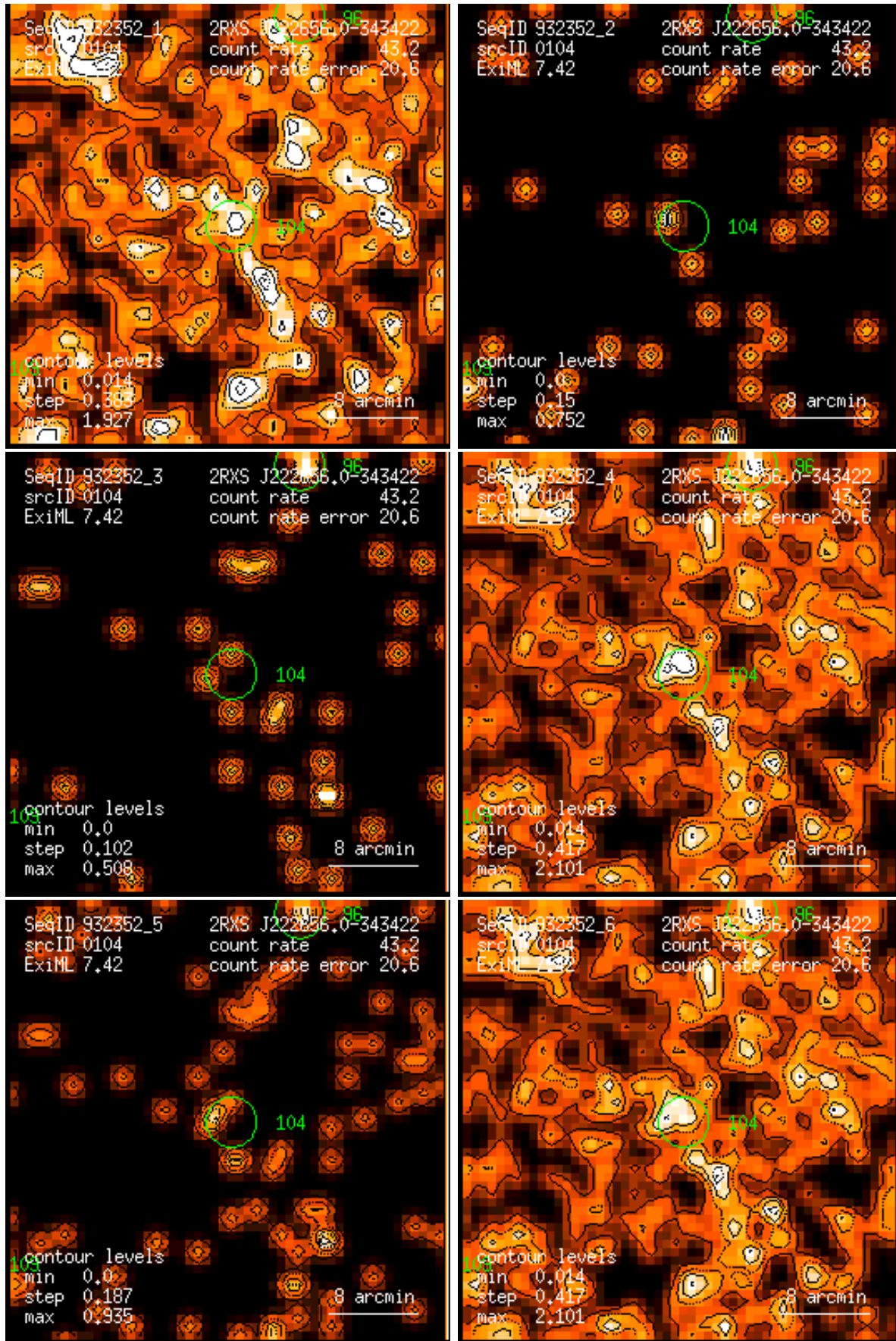
Figure 104: RASS 932352: detection 0104: band rate images, Gaussian filter: (1) PSPC channels 11 – 41, (2) 52 – 90, (3) 91 – 201, (4) 11 – 235, (5) 52 – 201, (6) 11 – 201. Broad band rates in counts/ks. Band rate contour levels in counts/ks/arcmin 2 .
