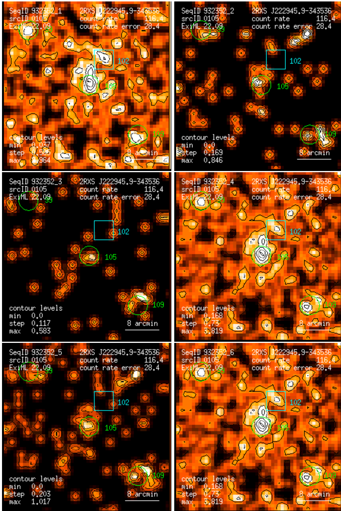
Figure 105: RASS 932352: detection 0105: band rate images, Gaussian filter: (1) PSPC channels 11 – 41, (2) 52 – 90, (3) 91 – 201, (4) 11 – 235, (5) 52 – 201, (6) 11 – 201. Broad band rates in counts/ks. Band rate contour levels in counts/ks/arcmin 2 .
