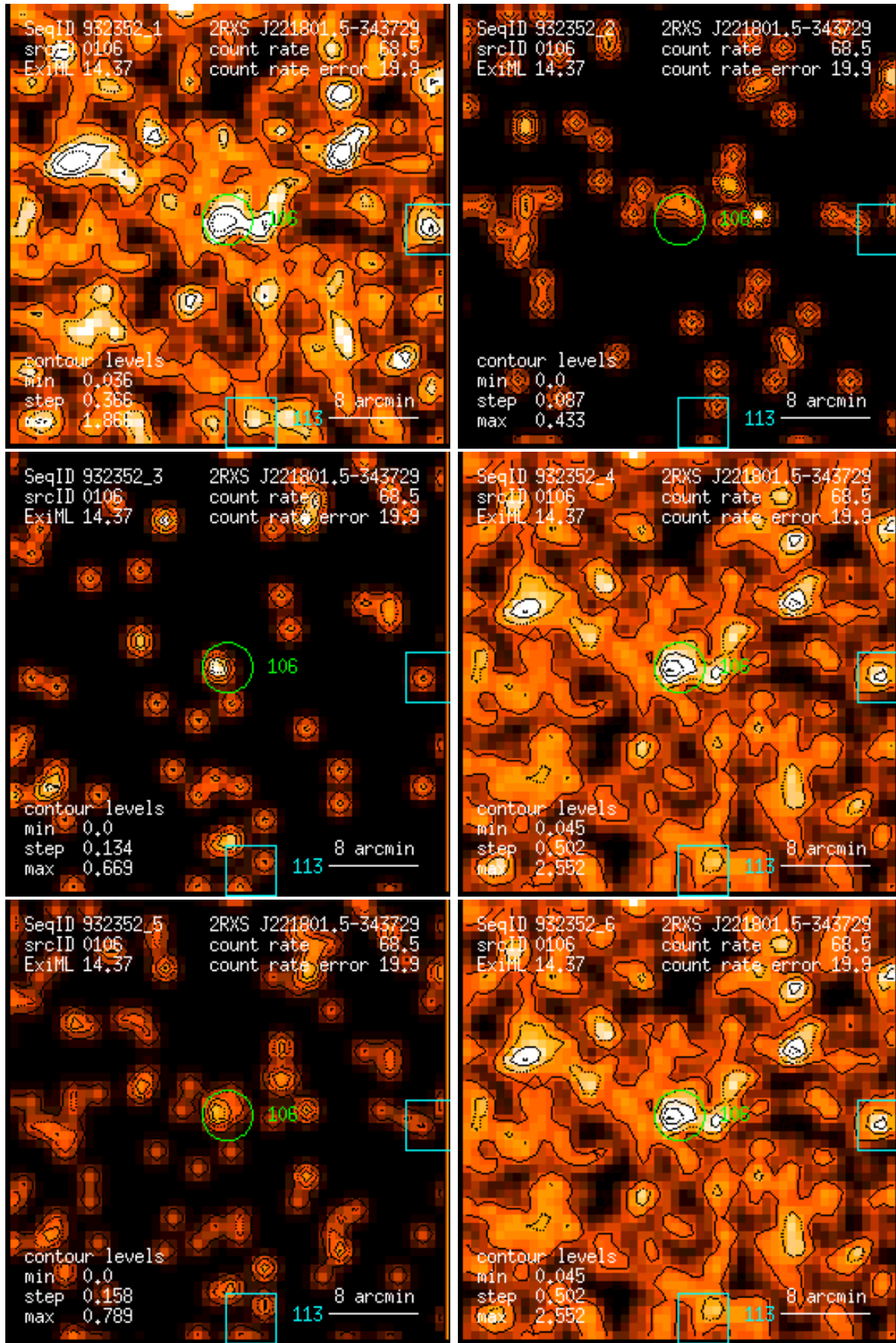
Figure 106: RASS 932352: detection 0106: band rate images, Gaussian filter: (1) PSPC channels 11 – 41, (2) 52 – 90, (3) 91 – 201, (4) 11 – 235, (5) 52 – 201, (6) 11 – 201. Broad band rates in counts/ks. Band rate contour levels in counts/ks/arcmin 2 .
