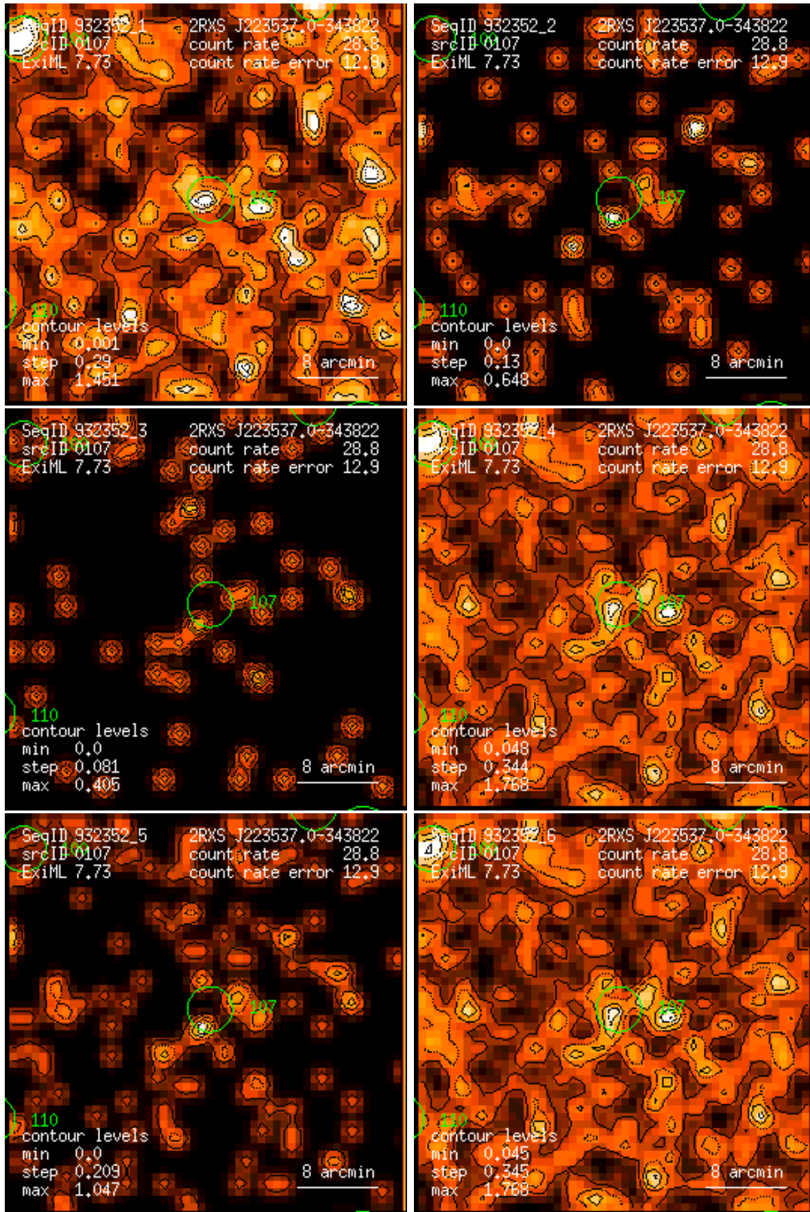
Figure 107: RASS 932352: detection 0107: band rate images, Gaussian filter: (1) PSPC channels 11 – 41, (2) 52 – 90, (3) 91 – 201, (4) 11 – 235, (5) 52 – 201, (6) 11 – 201. Broad band rates in counts/ks. Band rate contour levels in counts/ks/arcmin 2 .
